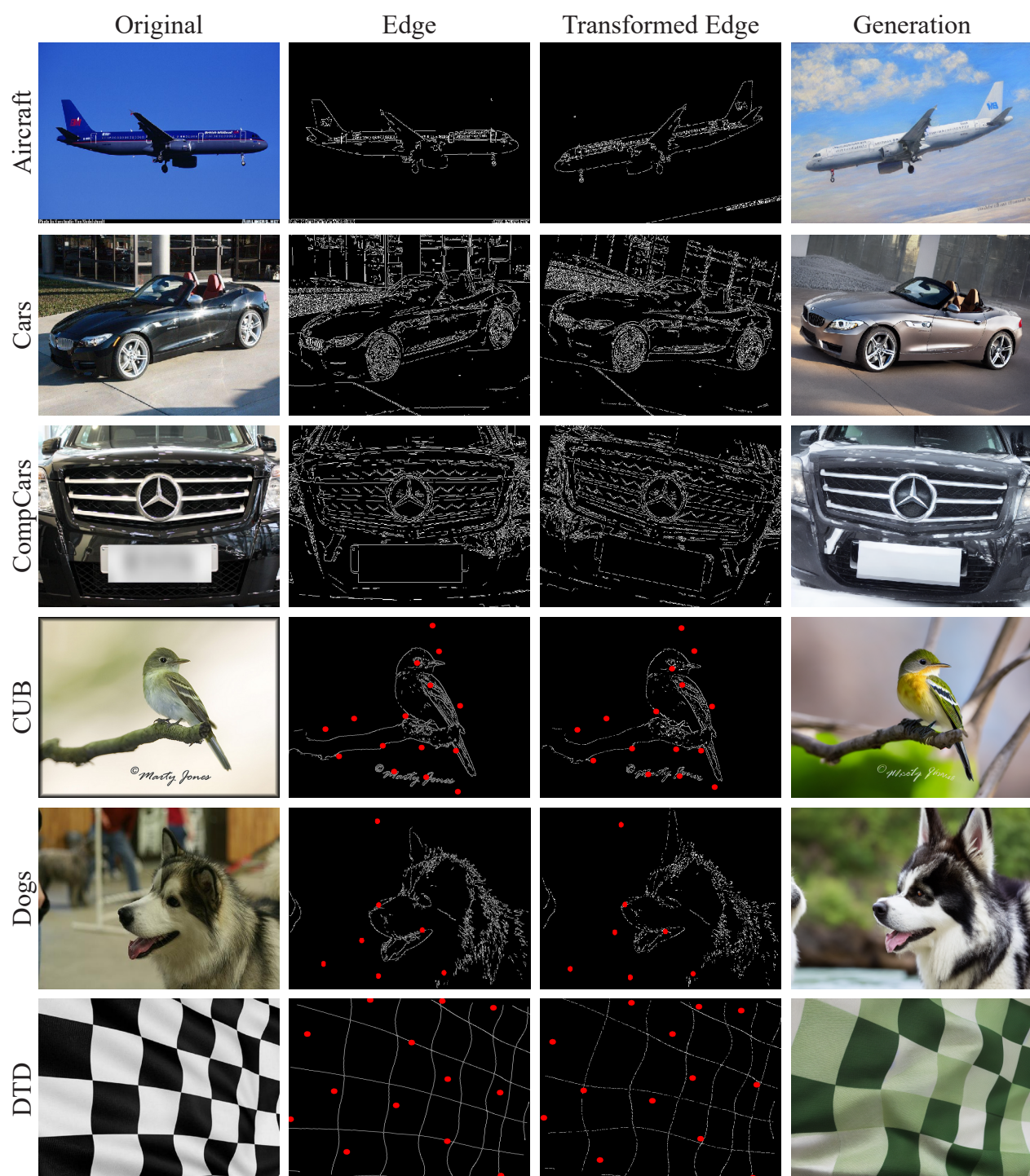
Figure 9: Examples of transformed contour images are shown. Random horizontal flipping and rotation modify object pose. The control points used for thin-plate spline interpolation are marked in the figure. By applying thin-plate spline interpolation, the shape can be modified. Transformations applied to contour maps help increase data diversity.
