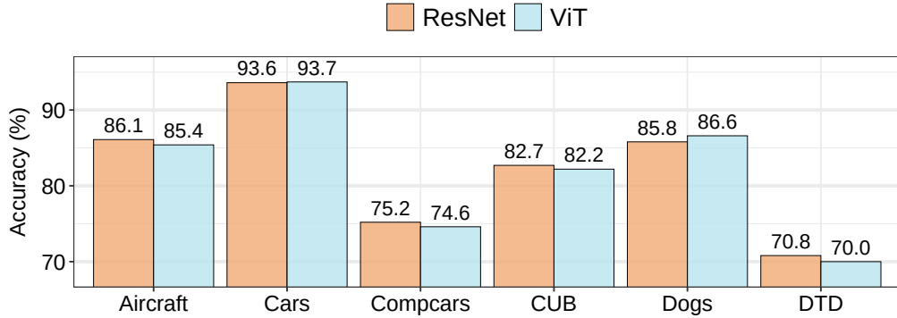
Figure 8: Comparison of Accuracy using the CAL classifier when HiGFA employs either a ResNet-50 or a ViT-B model for its internal feature guidance. The results show high similarity, indicating robustness to the choice of guidance architecture.
