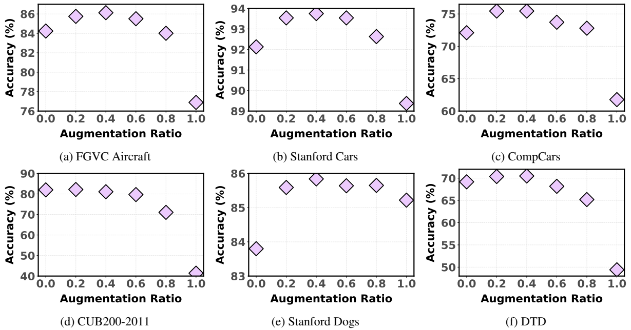
Figure 7: Impact of varying the augmentation ratio on accuracy across six datasets. The ratio represents the proportion of synthetic images generated by HiGFA within the combined training set. Accuracy is measured using the CAL classifier.
