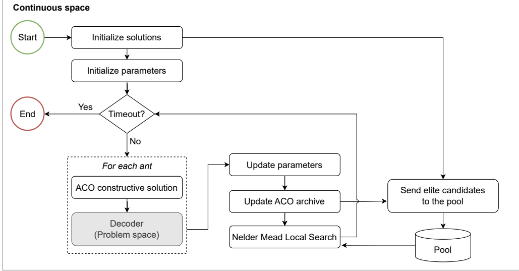
Figure 1: RKO-ACO flowchart
