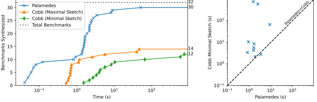
Fig. 19. Comparing PALAMEDES and Cobb. Left: Number of generators synthesized by PALAMEDES and Cobb over time (higher is better). Right: Per-benchmark comparison for the 10 benchmarks that both successfully synthesize (above the line means PALAMEDES is faster). Time axes are logarithmic.
