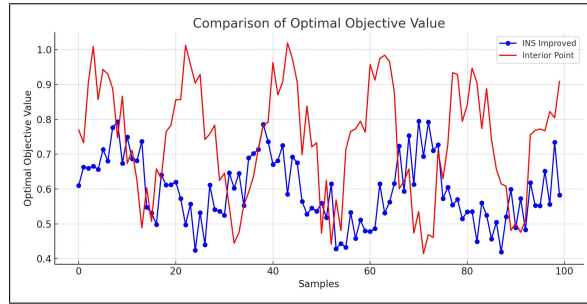
FIGURE 1. Comparison of the optimal value of the objective function
