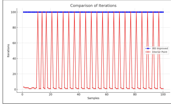
FIGURE 2. Comparison of the number of iterations
