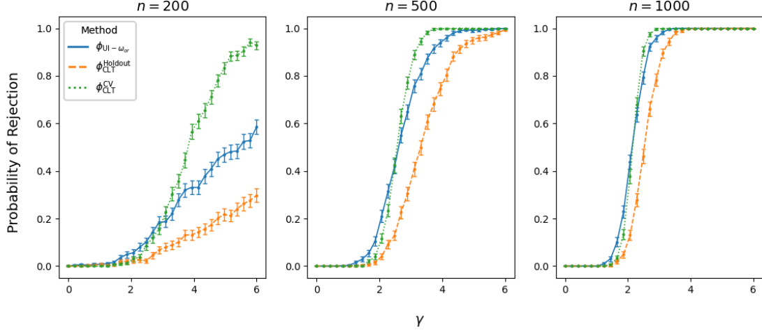
Figure 1: Rejection probabilities estimated across 1,000 simulations for various tests in the nonlinear regression setting with nominal level \alpha = 0.05 . The solid, dashed, and dotted lines correspond to the tests \phi_{UI-\omega_{or}} , \phi_{CLT}^{Holdout} , and \phi_{CLT}^{CV} , respectively. The bars correspond to estimated 95% confidence intervals for the power. We estimate the oracle choice of \omega_{or} from the data generating process when \gamma = 0 .
