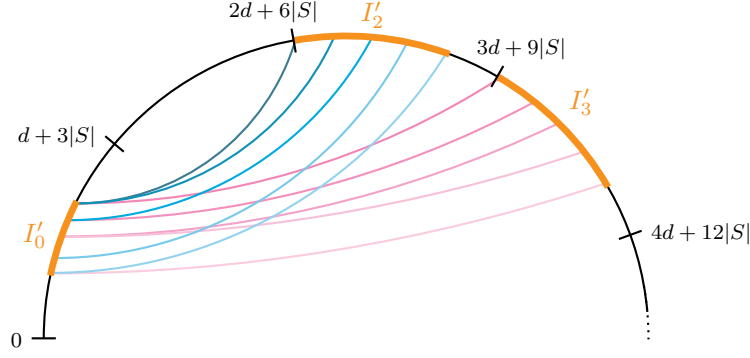
Figure 4: Intervals I_0, \dots, I_3 depicted around the semi-circle, with subintervals I'_0, I'_2 and I'_3 highlighted in orange. Vertices in S are embedded into I'_0 . In this example, v is adjacent to the vertices labelled by 2 and by 3 in T_{\text{aux}} , and we embed the root vertices corresponding to these vertex sets into I'_2 and I'_3 respectively. Blue edges have a colour in C_{02} , and lighter blue edges have larger colours than darker blue edges. The same holds for pink edges having colours in C_{03} .
