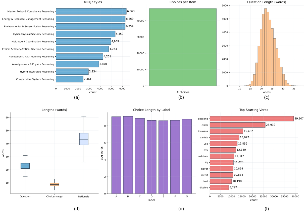
Fig. 3: Overview of UAVBench_MCQ dataset structure and linguistic statistics. (a) Distribution of multiple-choice question (MCQ) styles across reasoning domains; (b) Number of answer choices per question; (c) Distribution of question lengths in words; (d) Comparison of word counts for questions, averaged choices, and rationales; (e) Average choice length by option label (A–G); and (f) The most frequent starting verbs in the choice text. Together, these subfigures summarize the content balance, linguistic complexity, and stylistic diversity of UAVBench_MCQ items.
