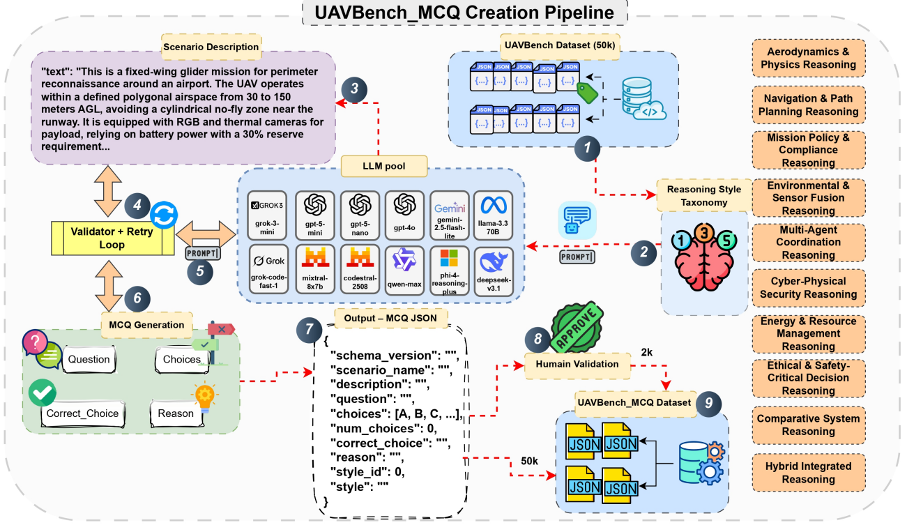
Fig. 4: UAVBench_MCQ Creation Pipeline.
