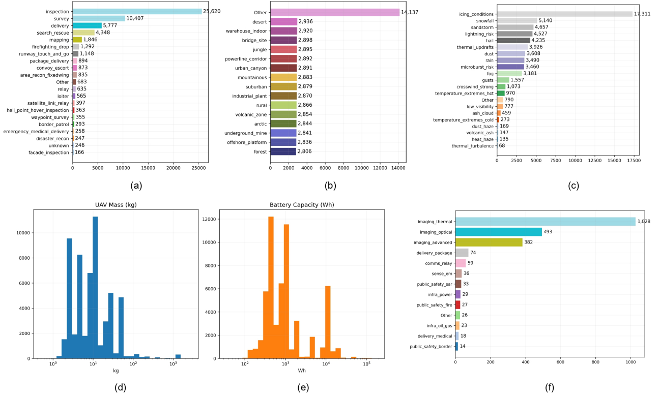
Fig. 2: Overview of UAVBench dataset composition and UAV design characteristics. (a) Mission types illustrating the diversity of operational scenarios; (b) Airspace types showing the range of environmental contexts; (c) Weather phenomena highlighting atmospheric complexity; (d) UAV mass distribution indicating variability in platform sizes; (e) Battery capacity distribution reflecting energy endurance profiles; and (f) Payload category frequencies summarizing the variety of onboard sensors and mission payloads.
