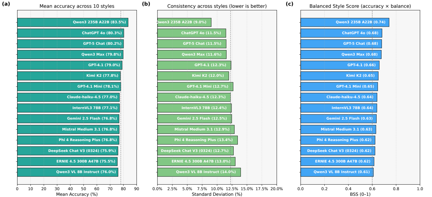
Fig. 5: Top 15 UAVBench_MCQ models ranked by Balanced Style Score (BSS). (a) Mean accuracy across ten reasoning styles, (b) cross-style consistency measured as the standard deviation of accuracies (lower is better; axis in %), and (c) BSS integrating both accuracy and consistency.
