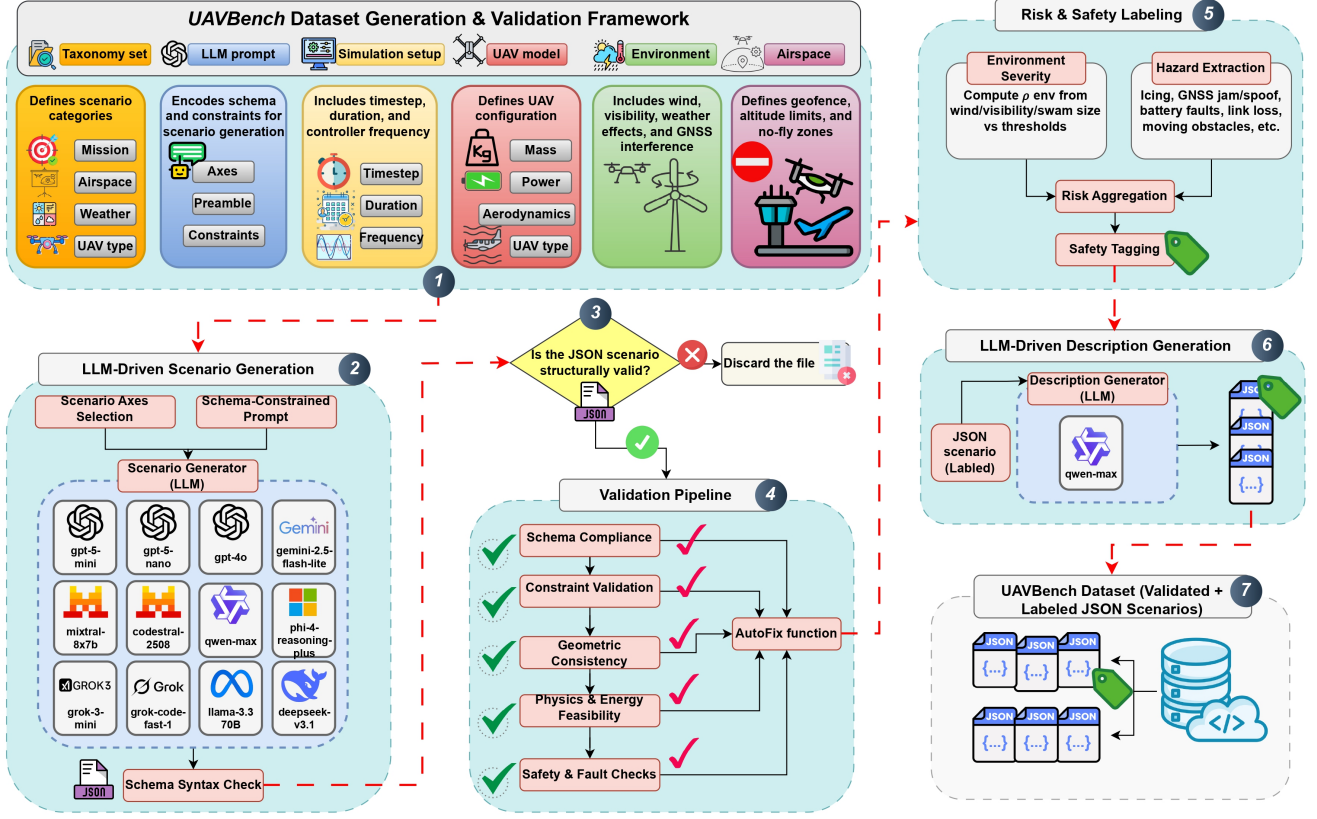
Fig. 1: UAVBench Dataset Generation, Validation, and Labeling Framework.
