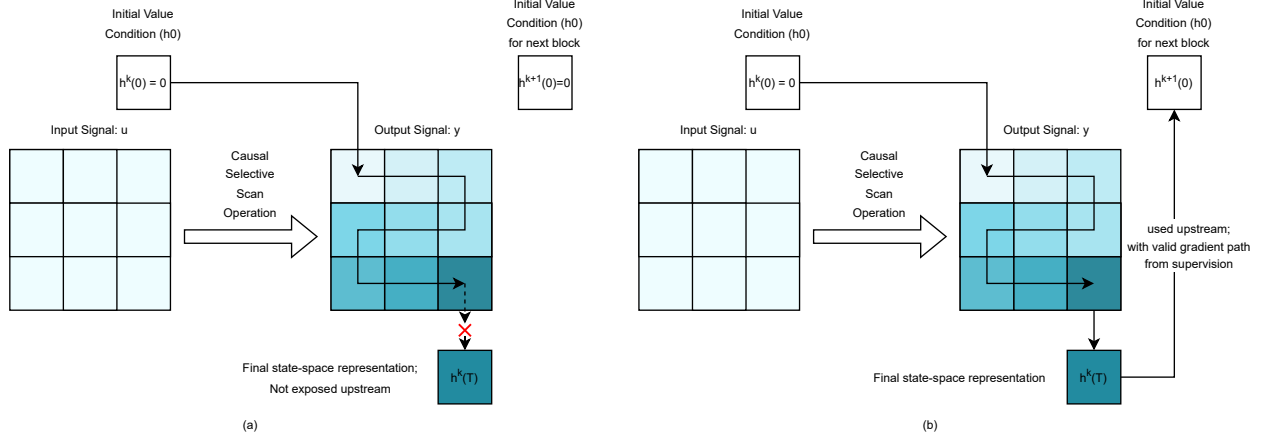
Figure 1. Conventional vs. Arcee selective scan. (a) In a vanilla Mamba block, the selective scan is strictly causal: the state is initialized with h^{(k)}(0) = 0 , the terminal state h^{(k)}(T) is discarded after producing y , and the next block again starts from zero. Darker cells indicate positions that have accumulated more context (later timesteps have seen a larger prefix of the sequence). (b) Arcee extends the scan to a two-port block: the terminal SSR h^{(k)}(T) is reused as the initial state h^{(k+1)}(0) of the next block via a differentiable boundary map, creating a recurrent state chain across depth with a valid gradient path and no change to the intra-block dynamics.
