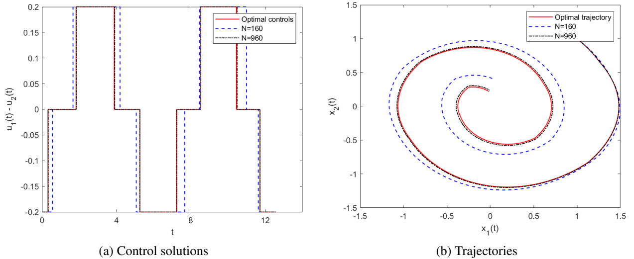
Figure 1: Red: optimal open-loop control and trajectory; Blue and Black: MPC generated solutions with N=160 and N=960 , correspondingly.
