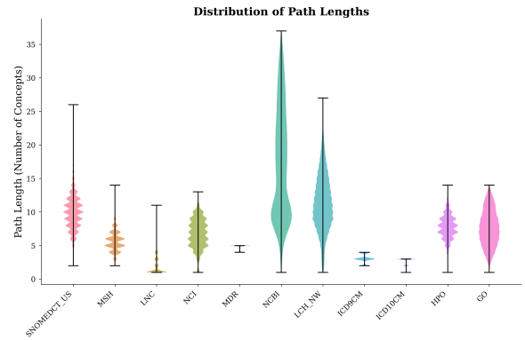
Figure 10: Path length distribution per vocabulary.
