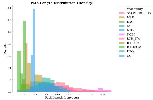
Figure 4: Histogram of lengths of entity hierarchical paths across different vocabularies.
