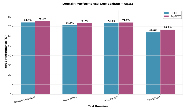
Figure 16: Performance of TF-IDF and SapBERT Candidate Generation across domains
