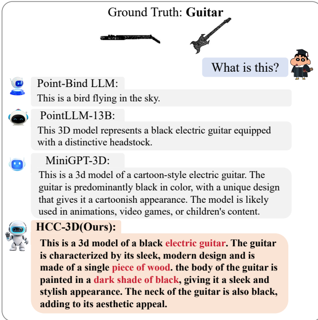
(a) 3D Object Recognition
