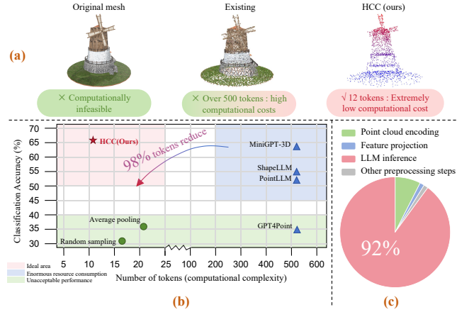
Figure 1: Performance comparison of 3D point cloud tokenization methods. (a) 3D Token Compression: HCC achieves 12 tokens vs. 500+ in existing Methods. (b) Relationship chart between token count and classification accuracy. Our HCC-3D uses less 3D tokens yet maintains higher performance. (c) Proportion of inference time. The LLM part of the current 3D VLMs takes over 90% computing costs. Best view in color.
