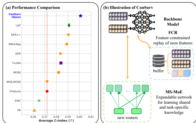
Figure 1: (a) Comparison of ConSurv against various CL methods on the MSAIL benchmark. (b) Illustration of ConSurv. It learns task-shared and task-specific multimodal knowledge during training with expandable MS-MoE, while consolidating previously acquired knowledge through FCR. A detailed architecture of ConSurv is presented in Figure 2.
