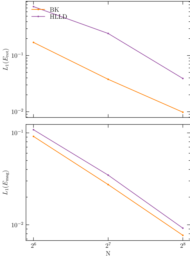
Figure A3. Variation of the L_1 norm with increasing resolution. N is the number of resolution elements in the x/y direction and L_E is calculated via Eq. (A4). USM-BK performs better than USM-HLLD and the error decreases with increasing resolution for both of them, implying that neither show any growth of dispersive errors, with M_{\text{cut}}/M = 2 is a good choice for USM-BK.
