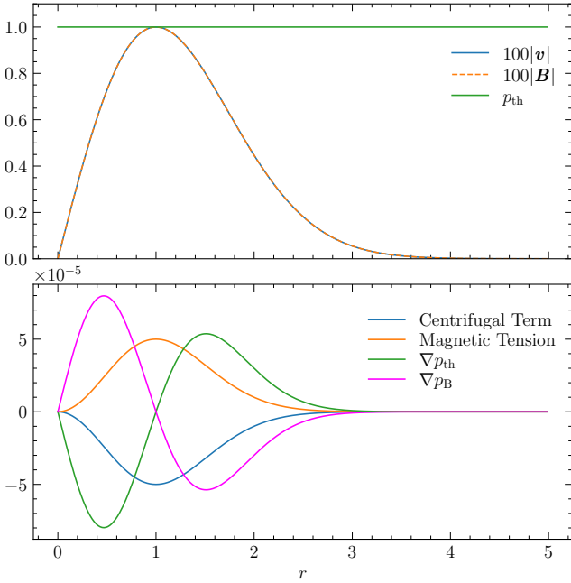
Figure 1. Top panel shows the radial profiles of velocity, magnetic field and pressure for the Balsara vortex, following Eqs. (16)–(18) for a sonic Mach number of \mathcal{M} = 0.01 and the ratio of the magnetic to the rotational kinetic energy \beta_k = 1 . Note that the velocity and magnetic pressure profiles have been scaled by a factor of 100 for the sake of clarity. The scaled velocity profile touches the thermal pressure profile ( p_{th} \approx 1 ) at r = 1 since \mathcal{M} = 0.01 . The bottom panel shows that the centrifugal term -(\mathbf{v} \cdot \nabla)\mathbf{v} is balanced by the magnetic tension (\mathbf{B} \cdot \nabla)\mathbf{B} , and the gradients of the thermal pressure ( \nabla p_{th} ) and the magnetic pressure ( \nabla p_B ) balance each other.
