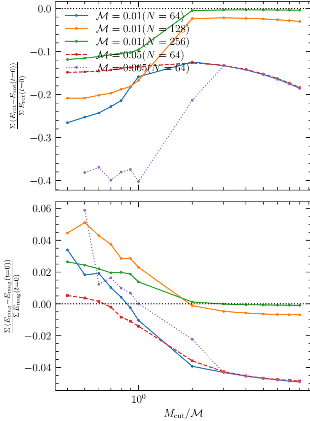
Figure A1. Variation of the amount of rotational (top panel) and magnetic energy (bottom panel) dissipated at the end of one advection as a function of M_{\text{cut}}/\mathcal{M} at various Mach numbers ( \mathcal{M}=0.005, 0.01, 0.05 ) and resolutions ( \mathcal{M}=0.01 at N=64, 128, 256 ). For M_{\text{cut}}/\mathcal{M} \leq 1 , there is a spurious increase in the magnetic energy and the dissipation of rotational energy. M_{\text{cut}}/\mathcal{M} \geq 1 provides a fairly universal choice that provides stable, physical solutions with low dissipation. We chose M_{\text{cut}}/\mathcal{M} = 2 for our 64 \times 64 test at Mach 0.01.
