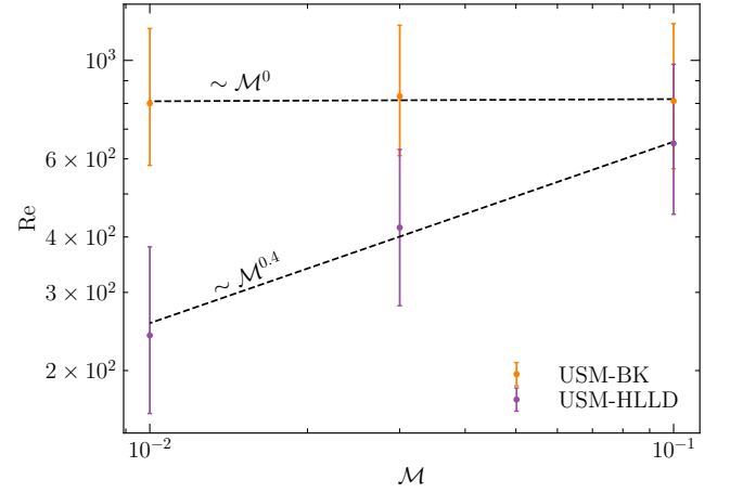
Figure 11. The effective numerical hydrodynamic Reynolds number ( \text{Re} ) as a function of the turbulent Mach number ( \mathcal{M} ). \text{Re} does not change with \mathcal{M} for USM-BK, however, it decreases with decreasing Mach number for USM-HLLD.
