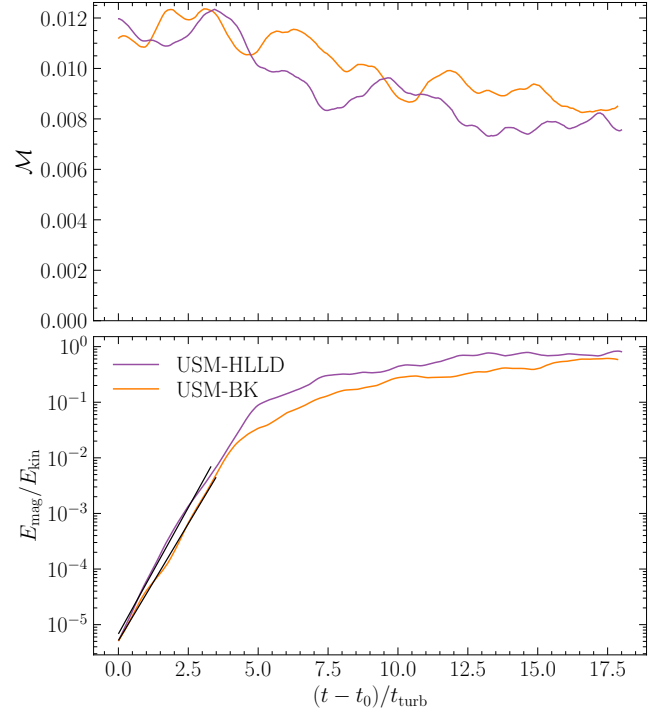
Figure 8. Similar to Fig. 5, but for Mach 0.01, comparing the best-performing solvers from the previous comparison at Mach 0.1, namely USM-BK (orange) and USM-HLLD (purple). Note that the x-axis shows (t - t_0)/t_{\text{turb}} , where t_0 is chosen such that both runs start at the same E_{\text{mag}}/E_{\text{kin}} to facilitate the comparison.
