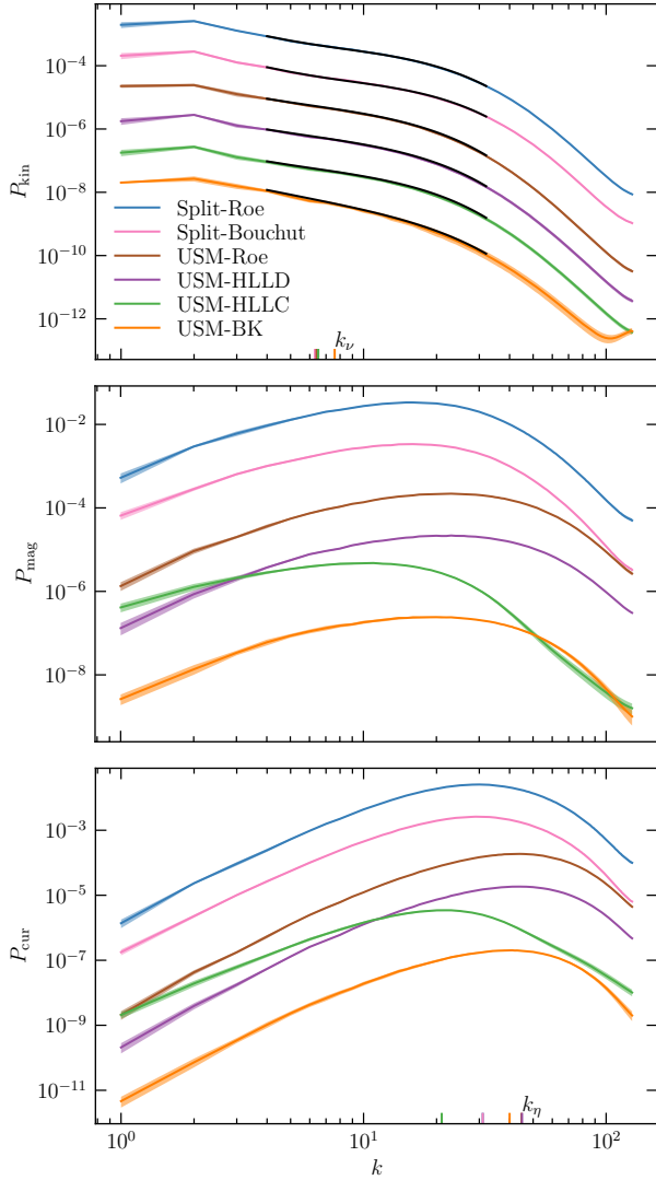
Figure 7. Time-averaged kinetic power spectra (top panel), magnetic power spectra (middle panel), and current power spectra (bottom panel) for various solvers. The spectra are multiplied for every solver except Split-Roe by a factor of 0.1 relative to the next solver in the legends. The black lines in the kinetic power spectra are the fits to the model given in Eq. (24). The viscous dissipation scale and resistive dissipation scale are marked on the x-axis. The viscous dissipation scales are clustered around each other for all solvers, however, the resistive dissipation scale measurements clearly show that HLLC is not suitable for MHD simulations since it is dissipative at very large length scales.
