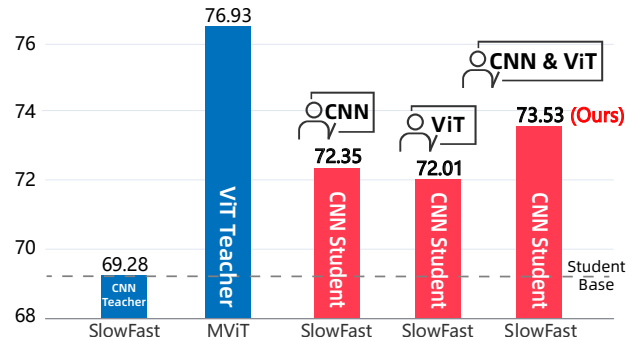
Figure 1: Motivation for our dual-teacher framework. A preliminary study shows that distillation from a weaker but structurally aligned CNN teacher can sometimes lead to better student performance than from a stronger, heterogeneous ViT teacher. This finding motivates the integration of both teacher types and highlights the critical role of architectural compatibility in cross-architecture knowledge transfer.
