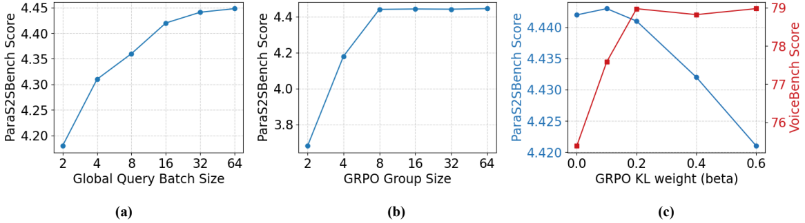
Figure 3 Ablating the effect of global batch size and GRPO’s group size and KL penalty weight. For all experiments, we optimize for the same number of steps.
