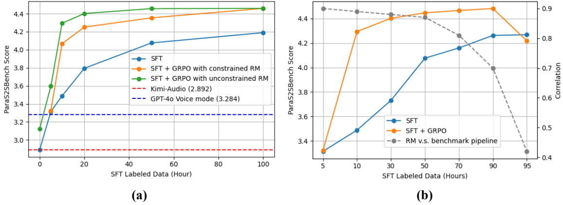
Figure 2 The ParaS2SBench score is the average across 4 categories. The trending of individual category is similar. (a) Comparison of RL and SFT results across different amounts of SFT data; (b) comparison of budget allocation between SFT and reward model (RM) data. The total budget consists of 100 hours of annotation, which are distributed between speech prompts for SFT data and reward model data. The gray dotted line shows the correlation between reward model prediction and the original benchmark pipeline score on a held-out test set.
