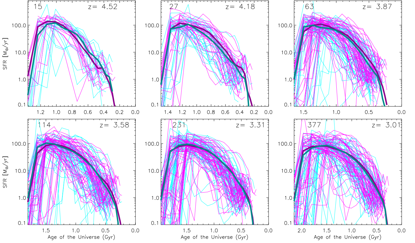
Fig. A.3. The star formation histories of galaxies in the bottom 25th (cyan) and highest 75th (magenta) percentiles of the distribution of \sigma_3 . Ticker lines show the median star formation histories. The numbers of galaxies in each sub-sample at each snapshot is given in the top left corner. A maximum of 50 individual star formation histories in each subsample is shown to avoid overcrowding the panels.
