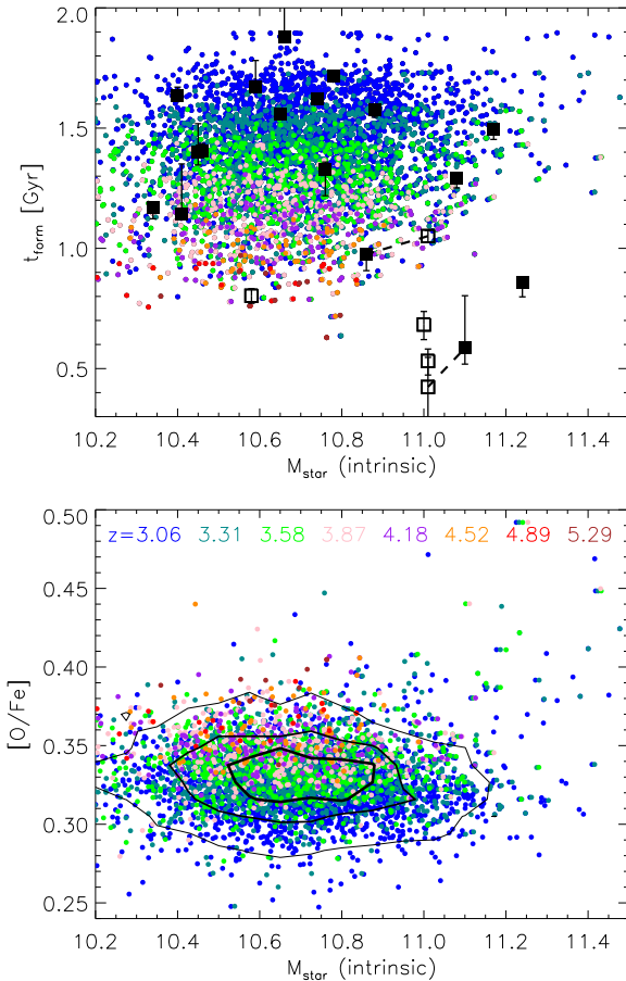
Fig. 6. Formation time (top panel) and [\text{O}/\text{Fe}] (bottom panel) as a function of galaxy stellar mass. The former is defined as the age of the Universe at which half of the stars in the galaxies are formed. Color coding is as a function of redshift, as indicated in the legend in the bottom panel. Open and filled symbols with error bars in the top panel correspond to observational measurements by Carnall et al. (2024, 5 galaxies between z \sim 3.2 and z \sim 4.6 ) and Nanayakkara et al. (2025, 19 galaxies with a median redshift of \sim 3.55 ), respectively. Contours in the bottom panel show the regions enclosing (from thicker to thinner) 30, 60, and 90 per cent of the model sample.
