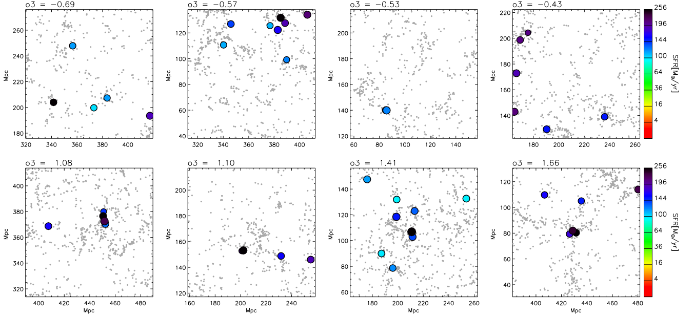
Fig. A.2. As in Fig. 3 but showing in colour only galaxies with star formation rates larger than \sim 80 M_{\odot} \text{ yr}^{-1} .
