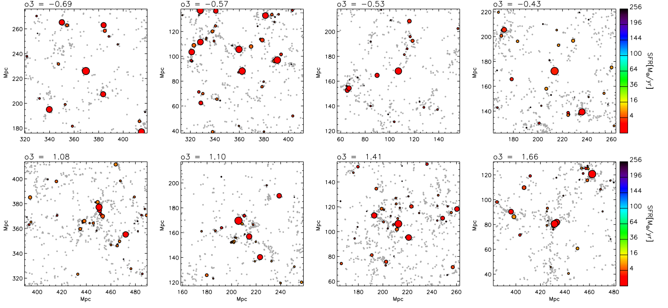
Fig. A.1. As in Fig. 3 but showing in colour only galaxies with star formation rates lower than \sim 5 M_{\odot} \text{ yr}^{-1} .
