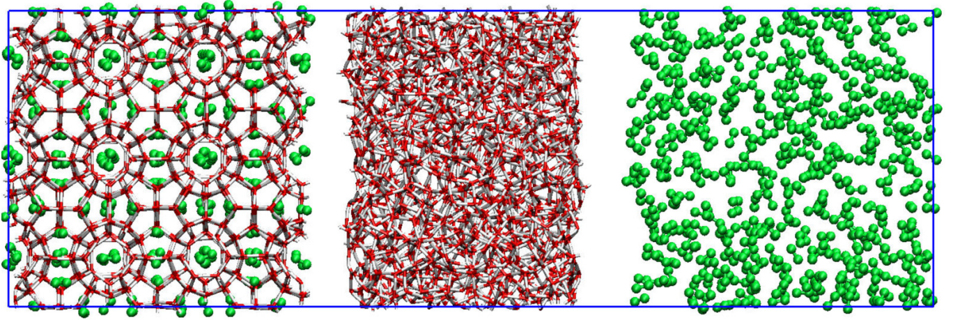
FIG. 1. Representation of the initial simulation box used in this work. green spheres represent the \text{C}_2\text{H}_6 molecules and red and white licorice representations correspond to water molecules. From left to right, the simulation box is conformed by a hydrate phase, a water phase, and a \text{C}_2\text{H}_6 phase.
