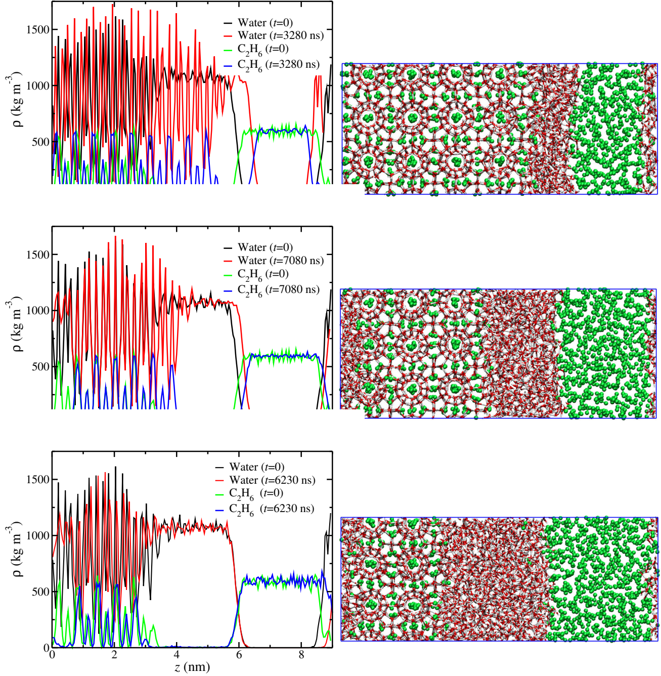
FIG. 4. Ethane and water density profiles and snapshots at 2500 bar at 308 (top), 310 (middle), and 312 K (bottom). The density profiles show the initial and final density distribution of water and \text{C}_2\text{H}_6 along the simulation box, while the snapshots show the final configuration obtained from the NPT simulations.
