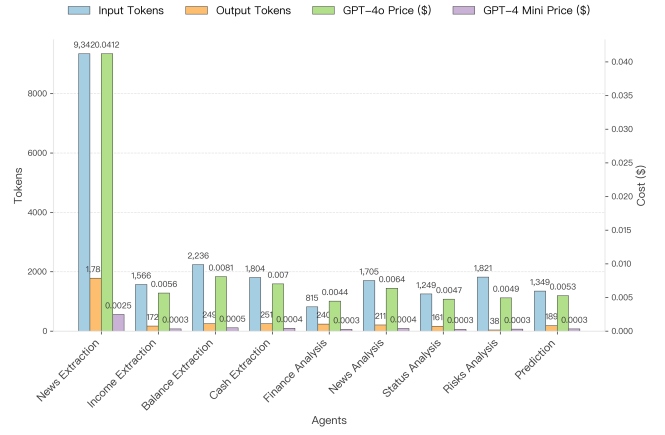
Figure 5: The average input tokens, output tokens, and costs for each agent. (The price calculation is based on the official API price of OpenAI as of February 1, 2025.)
