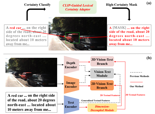
Figure 1: (a) Existing methods over-rely on high-certainty words (e.g., “red car”) within descriptions (left), causing spatial description neglect. Our CLIP-LCA dynamically masks such high-certainty words during training, forcing the text encoder to comprehend spatial descriptors; (b) Previous methods employ generalized textual features (containing both 2D and 3D information) to refine both 3D visual (depth) features and 2D visual features, causing cross-dimensional interference. We propose D2M to decouple dimension-specific text features (2D and 3D separately) for dimensionally-consistent cross-modal interactions.
