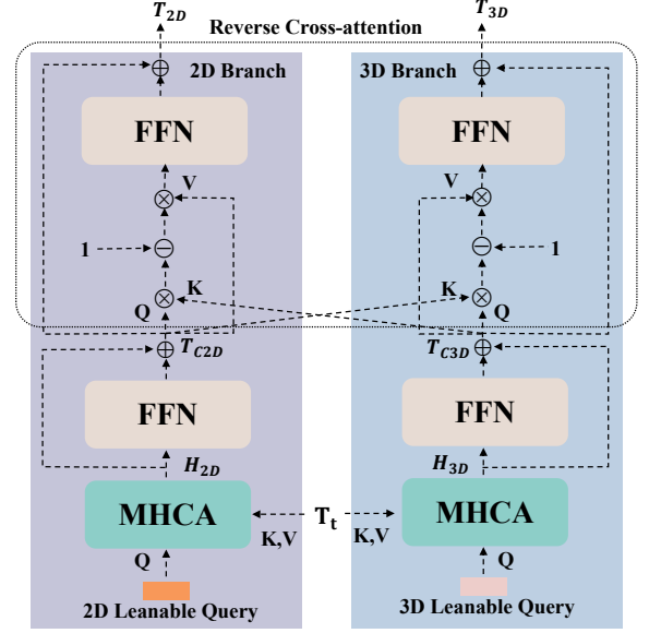
Figure 3: The detailed architecture of Dimension-Decoupled Module. The left part illustrates the procedure for decoupling 2D-specific textual features T_{2D} , while the right section presents the corresponding workflow for 3D-specific textual features T_{3D} .
