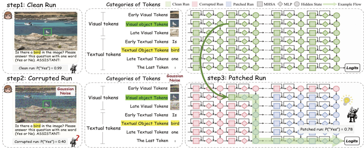
Figure 2: Overview of our proposed Fine-grained Cross-modal Causal Tracing method. Activation patching computes the causal effect of a specific component by running the LVLMs three times: a clean run (step1) with original image, a corrupted run (step2) with image added Gaussian noise, and a patched run (step3) with corrupted input but restoring specific component using the value in the clean run. We use Recovery Rate to quantify the causal effect of each restored component.
