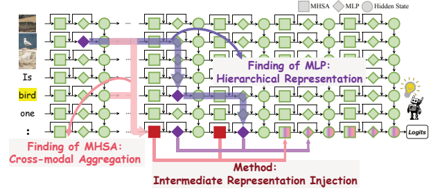
Figure 1: An overview of our proposed Fine-grained Cross-modal Causal Tracing (FCCT) findings and Intermediate Representation Injection (IRI) method.
