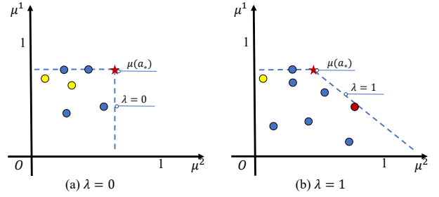
Figure 1: Cross-objective Acceleration
