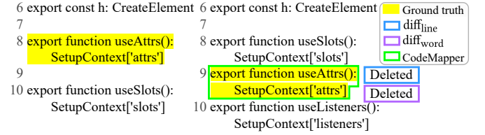
Figure 6: A source region involved in a vertical movement. Only CodeMapper finds an exact match of the target region.
