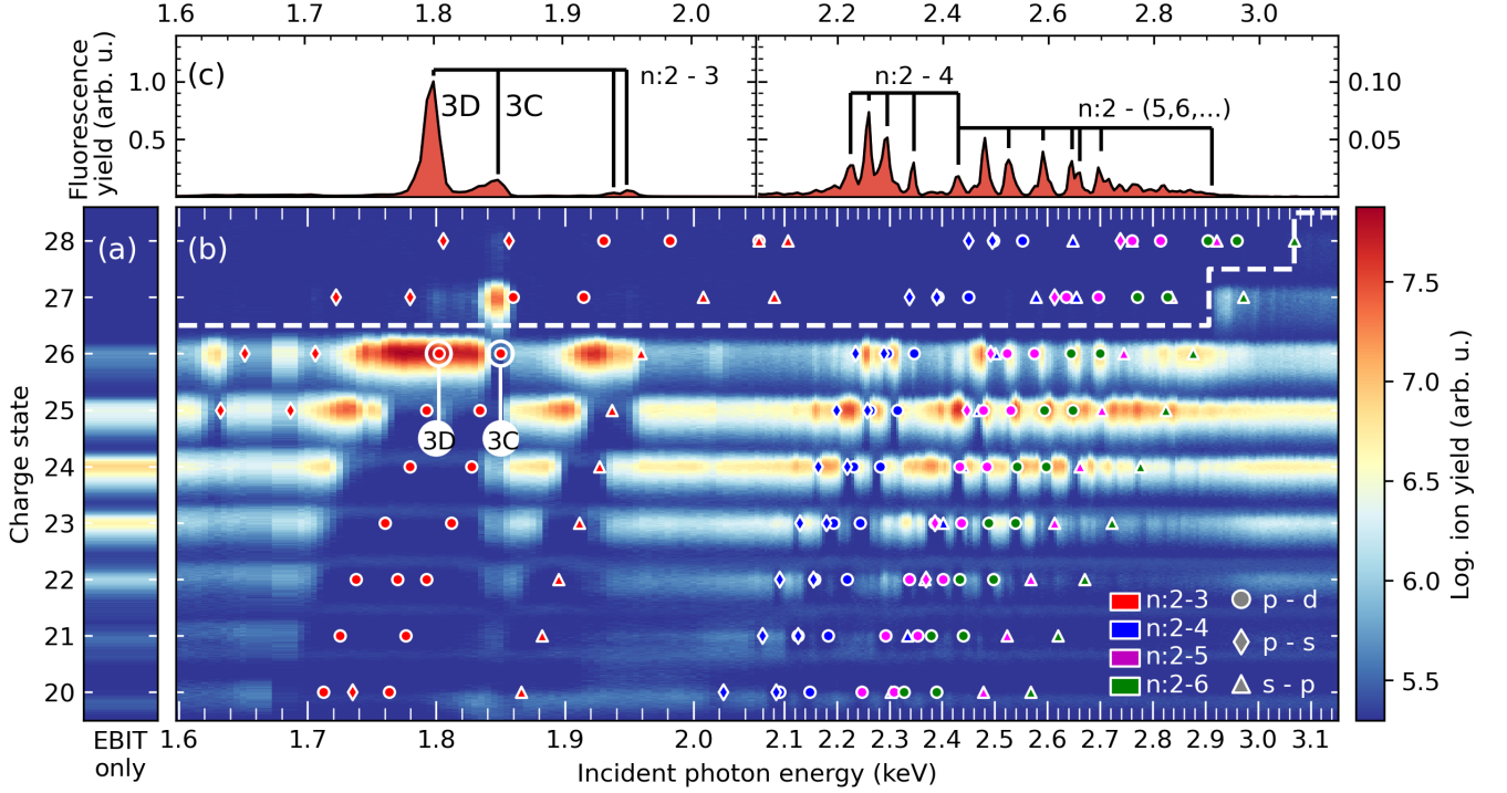
FIG. 3. Overview spectrum from 1.6 keV to 3.1 keV with highly charged krypton in EBIT. (Top) Fluorescence yield; (bottom) charge-state distribution (CSD) versus incident photon energy; (left) initial CSD without XFEL irradiation. Note the change in the scaling of the photon-energy axis around 2.1 keV. Predicted energies of major ground-state transitions for each charge state are marked with colors according to the upper state n and symbols for the orbital angular momentum, e.g., blue circles for 2p \rightarrow 4d transitions. The white dashed line marks the ionization threshold.
