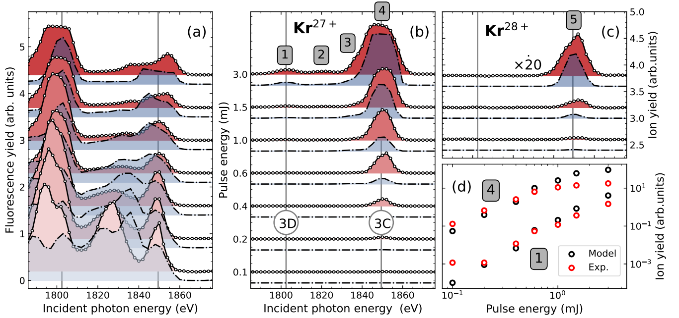
FIG. 4. Experimental data (red) and predictions (grey) for the photon energies near the 3C and 3D resonant transitions for varying pulse energy. (a): Average fluorescence yield. (b): ion-yield spectra for fluorine-like krypton. (c): ion yield spectra for oxygen-like krypton. Five identified peaks are labeled from 1 to 5. (d) Comparison of \text{Kr}^{27+} yield evaluated at 1800 eV (peak (1)) and 1850 eV (peak (4)) as a function of the pulse energy.
