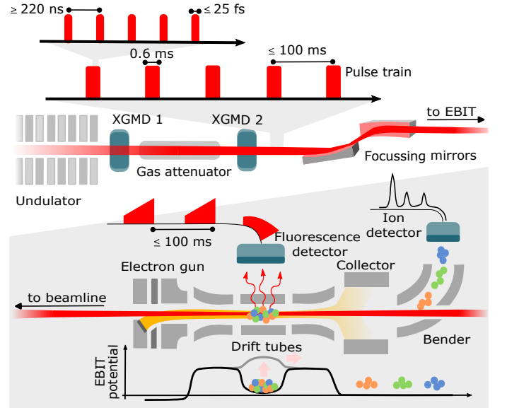
FIG. 2. Top: Scheme of the SASE3 beamline at EuXFEL. XFEL pulses with the depicted pattern from an undulator pass XGMD1 (for intensity measurements), a gas attenuator and a second intensity monitor (XGMD2). Two KB mirrors focus the beam into the experimental chamber (bottom) of SQS-EBIT to irradiate HCIs produced and trapped in it. A silicon drift detector records their fluorescence, while an ion-ToF spectrometer downstream of the EBIT registers their charge-state distribution after each exposure period. The bottom panel depicts the electrostatic potential of EBIT and ion extraction beamline.
