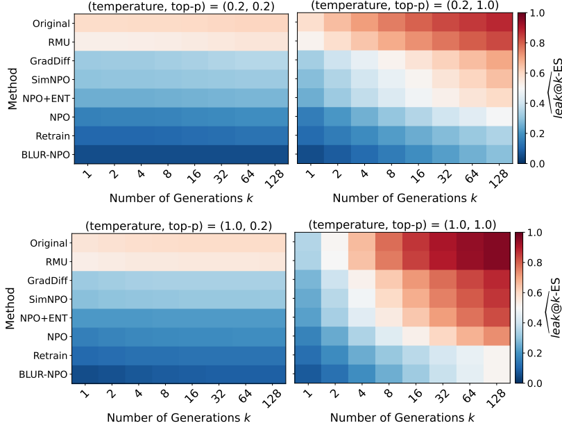
Figure 2: \widehat{\text{leak}}@k\text{-ES} heatmaps for unlearning methods on the TOFU benchmark with LLaMA-3.2-1B. Each cell reports ES across k generations. Rows denote unlearning methods, columns denote values of k , and each plot corresponds to a different (\text{temperature}, \text{top-}p) configuration. Leakage is almost stable at (0.2, 0.2) but increases with larger p values, even when temperature remains low, whereas high T with low p does not produce explicit leakage.
