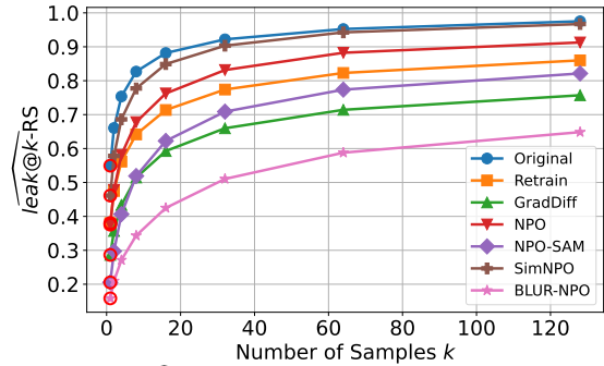
Figure 1: \widehat{\text{leak}@k} measure using ROUGE-L score ( \widehat{\text{leak}@k}\text{-RS} ) for various unlearned models on MUSE-News dataset using LLaMA2-7B model at T=0.2 and p=1.0 . When k is small, the unlearned models show limited leakage in providing information from the forget set. However, as k increases, all models reveal increasingly sensitive information about the forget set questions.
