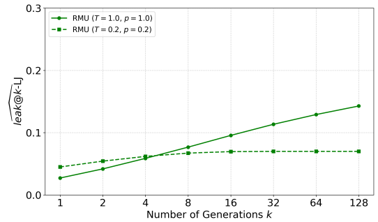
Figure 6: \widehat{\text{leak@}k\text{-LJ}} for RMU under two decoding settings (T, p) = (0.2, 0.2) and (T, p) = (1.0, 1.0) . RMU shows minimal information leakage under low randomness but exhibits a clear leakage trend under high-randomness decoding, consistent with the behavior observed for \widehat{\text{leak@}k\text{-Acc}} .
