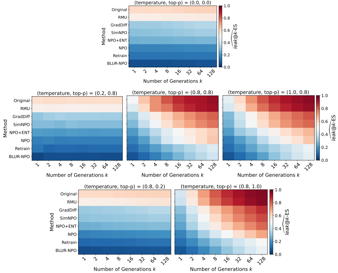
Figure A1: \widehat{\text{leak}}@k\text{-ES} heatmaps for unlearning methods on the TOFU benchmark with LLaMA-3.2-1B. Each cell reports ES across k generations. Rows denote unlearning methods, columns denote values of k , and each plot corresponds to a different (\text{temperature}, \text{top-}p) configuration.
