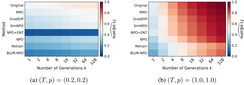
Figure 3: \widehat{\text{leak}}@k\text{-LJ} heatmaps for unlearning methods on the TOFU benchmark with LLaMA-3.2-1B using two sampling configurations (T, p) = (0.2, 0.2) and (T, p) = (1.0, 1.0) . A slight rise appears at low randomness, while LJ confirms explicit information leakage under high-randomness decoding.
