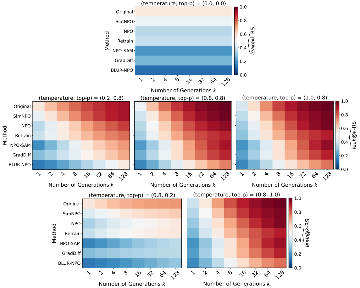
Figure A3: \widehat{\text{leak}}@k\text{-RS} heatmaps for various unlearning methods evaluated on the MUSE-News benchmark using the LLaMA2-7B model. Each heatmap cell represents ROUGE-L recall achieved across k generations. Rows correspond to different unlearning methods, and columns represent the number of generations k . Each plot varies in sampling configuration (temperature, top- p ).
