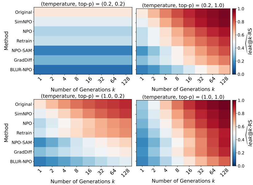
Figure 4: \widehat{\text{leak}}@k\text{-RS} heatmaps for various unlearning methods evaluated on the MUSE-News benchmark using the LLaMA2-7B model. Each heatmap cell represents ROUGE-L recall achieved across k generations. Rows correspond to different unlearning methods, and columns represent the number of generations k . Each plot varies in sampling configuration (temperature, top- p ).
