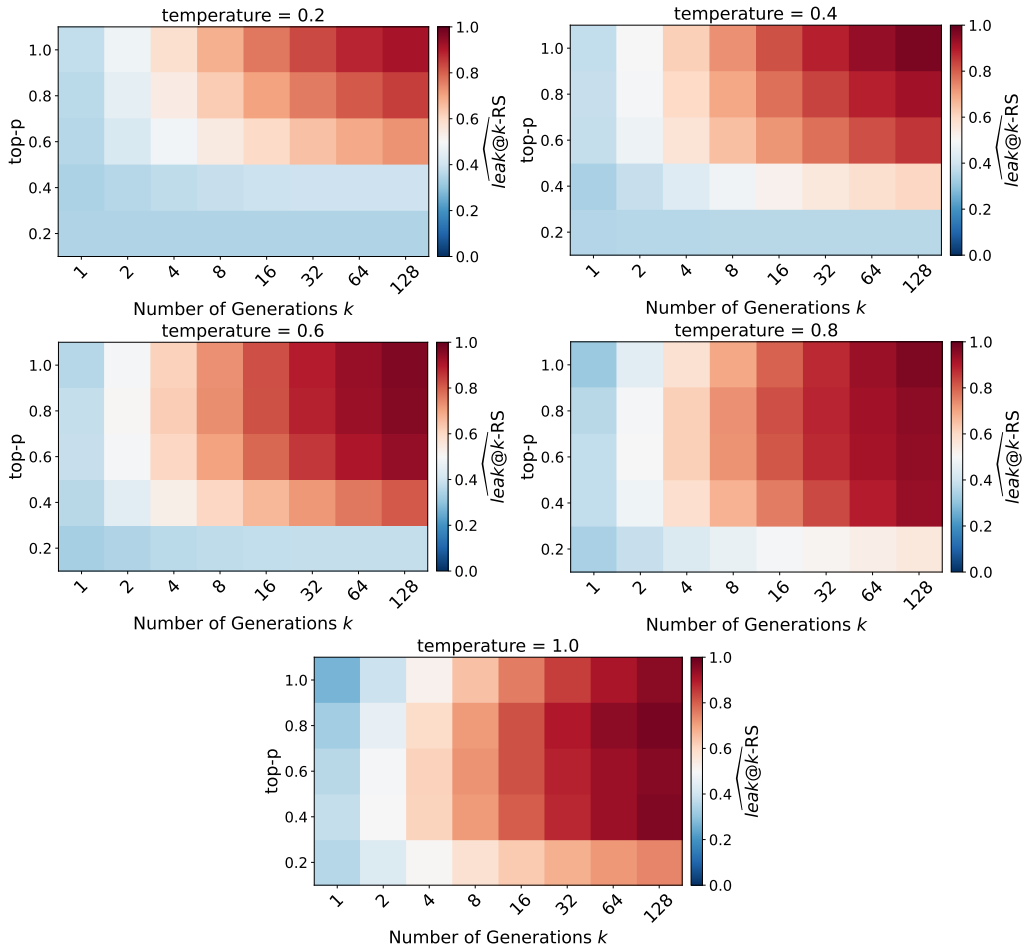
Figure A5: Heatmaps of \widehat{\text{leak@}k\text{-RS}} for the NPO model on the MUSE-News benchmark using the LLaMA2-7B model. For each fixed temperature T \in \{0.2, 0.4, 0.6, 0.8, 1.0\} , rows show results across \text{top-}p \in \{0.2, 0.4, 0.6, 0.8, 1.0\} and columns correspond to the number of generations k .
