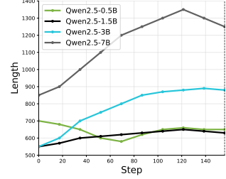
Figure 3: Comparison of average response length over the training steps.
