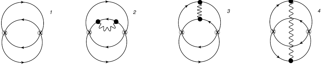
FIG. 2. Feynman diagrams contributing to \langle \mathcal{O}_{\Gamma\bar{\Gamma}}(x) \mathcal{O}_{\Gamma'\bar{\Gamma}'}^\dagger(y) \rangle , to order \mathcal{O}(g^0) (diagram 1) and \mathcal{O}(g^2) (the remaining diagrams). Wavy (solid) lines represent gluons (quarks). Diagrams 2 and 4 have also mirror variants.
