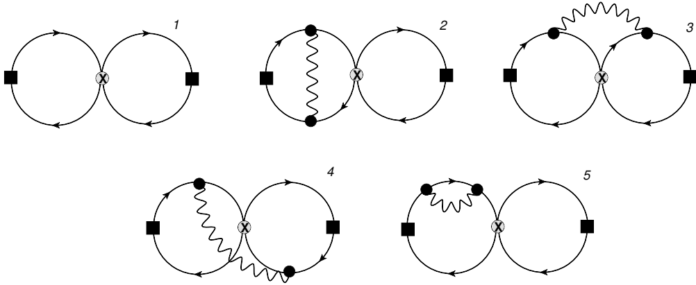
FIG. 3. Feynman diagrams contributing to \langle \mathcal{O}_{\Gamma'}(x) \mathcal{O}_{\Gamma\bar{\Gamma}}(0) \mathcal{O}_{\Gamma''}(y) \rangle , to order \mathcal{O}(g^0) (diagram 1) and \mathcal{O}(g^2) (the remaining diagrams). Wavy (solid) lines represent gluons (quarks). A circled cross denotes the insertion of the four-quark operator, and the solid squares denote the quark bilinear operators. Diagrams 2-5 have also mirror variants.
