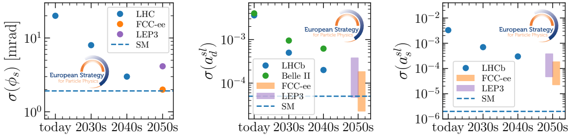
Fig. 5.12: Current and expected precision on the CPV phase \phi_s (left) and the semileptonic asymmetries a_d^s (middle) and a_{sl}^s (right) which characterise CPV in B^0 and B_s^0 mixing.
