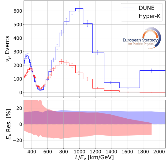
Fig. 6.2: Oscillated muon neutrino spectrum in Hyper-K and DUNE after 10 years running (top). An estimation of their energy resolution, considering only nuclear effects using, respectively, NEUT 5.8.0 and GENIE V3 (bottom). For DUNE (Hyper-K) charged current events (without pions) are considered.
