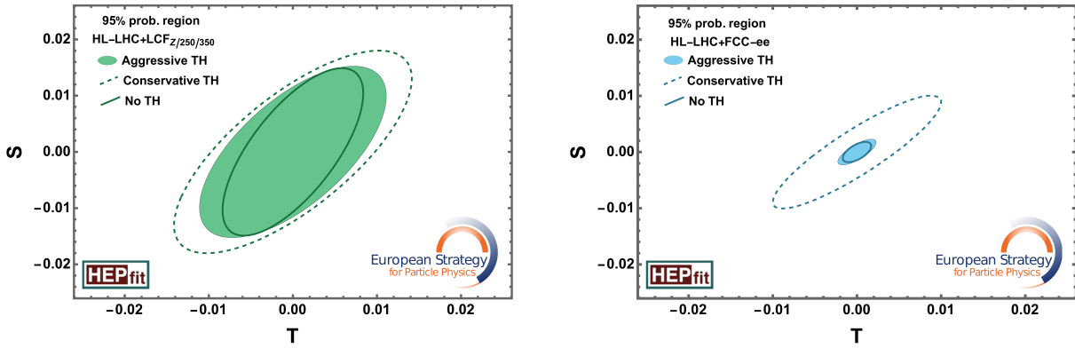
Fig. 3.4: The oblique parameters S and T shown with various theory comparisons for the LCF (left panel) and FCC-ee (right panel).
