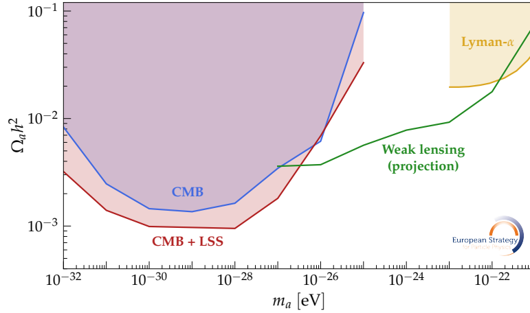
Fig. 9.1: The allowed parameter space for the energy density in ULDM as a function of mass. Shaded regions correspond to current bounds, while the lines display projections for datasets that will come online within the next decade.
