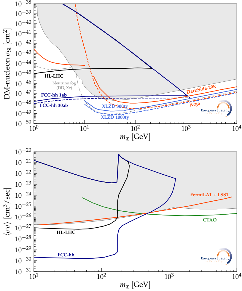
Fig. 9.6: Collider limits for (top) scalar and (bottom) pseudo-scalar models compared to direct and indirect constraints, respectively—see text for references. The grey area represents current constraints from direct detection experiments. Future projections for XLZD [713] and DarkSide [718] are overlaid. The notebook to generate the figures is available at [660].
