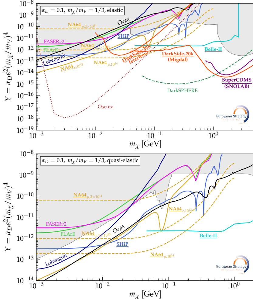
Fig. 9.4: Parameter space of elastic (top) and quasi-elastic (bottom) DM models with the dark photon mediator, in the plane m_\chi - Y , with Y = \epsilon^2 \alpha_D (m_\chi/m_V)^4 . The model parameters are \alpha_D = 0.1, m_\chi/m_V = 1/3 and in the quasi-elastic case the splitting is small, but sufficient to suppress direct detection signatures. The thick black line “ \Omega_{\text{DM}} ” corresponds to the parameter space where the model explains the DM abundance in the standard scenario. The grey shaded constraints come from the combination of accelerator and DM direct detection probes [645, 656, 672, 707]. NA64 sensitivity [672] comes from the invisible dark photon decay signature. The SBND experiment also has sensitivity to these models, but existing projections [708] require knowing background status for interpreting them.
