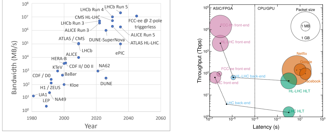
Fig. 11.3: Left: Evolution of data rates over time for large high-energy physics experiments. (Source: A. Cerri (Università di Siena & INFN Pisa), D. vom Bruch (CPPM & Aix Marseille University)) Right: Characteristic throughput versus latency for real-time processing systems. Event sizes for FCC-hh and FCC-ee are approximate, based on reference detectors [896, 995]. LHC and HL-LHC data are from CMS/ATLAS. Packet size is the unit size of transmitted data (e.g., event size in colliders; movie, image, or webpage size in industry). (Source: T. Aarrestad (ETH Zurich), S. Summers (CERN))
