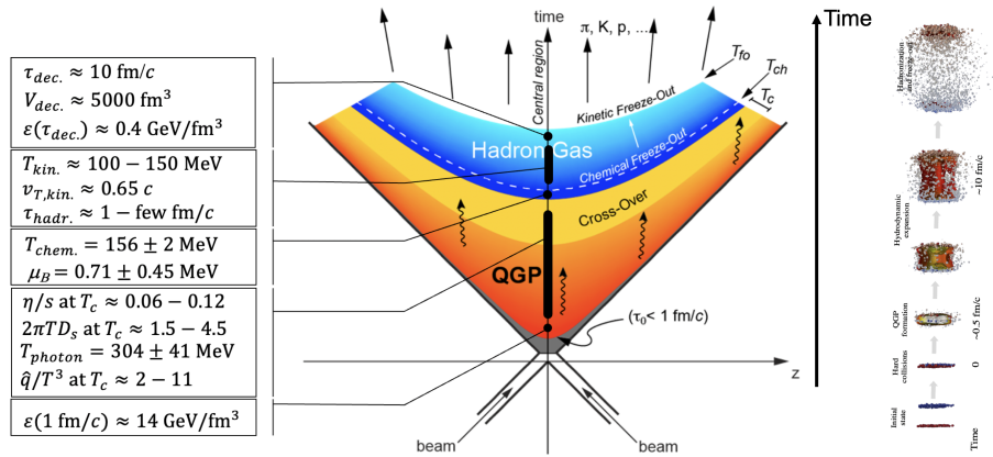
Fig. 4.5: Time evolution of the QGP formed in heavy-ion collisions, with numerical values estimated on the basis of LHC measurements or their model description. Figure from [123].
