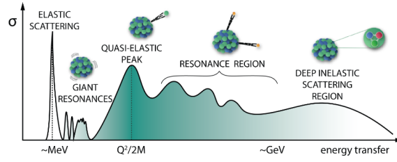
Fig. 6.6: A qualitative overview of the evolution of the neutrino-nucleus inclusive interaction cross-section as a function of energy transfer for a fixed scattering angle (from [ID135]).
