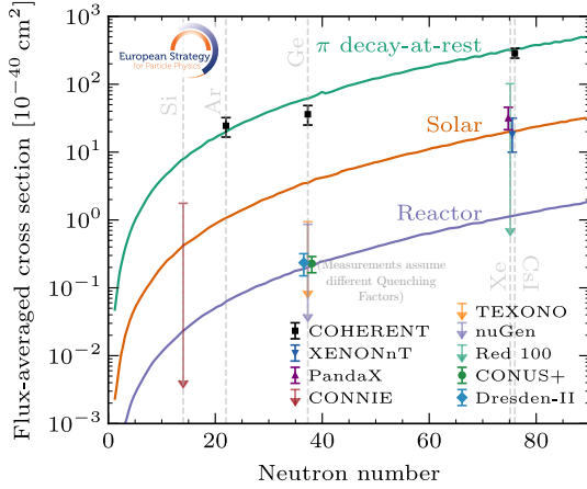
Fig. 6.5: Current CEvNS measurements
