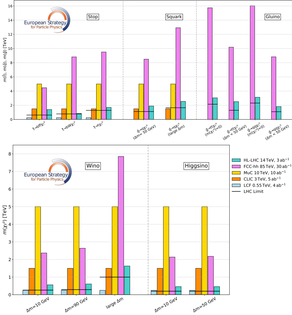
Fig. 8.5: Projected 95% exclusion limit for strongly interacting (top) and weakly-only interacting particles (bottom) as a function of their mass in a LSP simplified model for representative decay modes. For stops: (i) Top quark+LSP with large stop-LSP mass splitting \Delta m . (ii) Bottom quark + W boson + LSP with m_W < \Delta m < m_t . (iii) Bottom quark + off-shell W boson + LSP with \Delta m < m_W . For light-flavour squarks: Quark + LSP, corresponding to (i) large squark-LSP mass splitting and (ii) with \Delta m = 50 GeV. For gluinos: (i) Top quarks + LSP, corresponding to large gluino-LSP mass splitting \Delta m . (ii) Off-shell top quarks + LSP with a compressed spectrum, \Delta m = 50 GeV. (iii) Light-flavor quarks + LSP, with large \Delta m . (iv) Light-flavor quarks + LSP with \Delta m = 50 GeV. For winos, decays into bino + electroweak bosons in three cases, compressed ( \Delta m = 10 GeV), moderately compressed ( \Delta m = 50 GeV) and large wino-bino mass splittings. For the higgsinos, decays of neutral and charged higgsino to lightest neutral higgsino, corresponding to compressed mass splittings \Delta m = 10 and 50 GeV.
