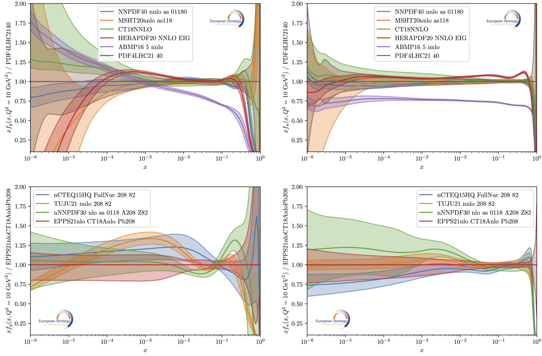
Fig. 4.3: Top : Comparisons of the uncertainties of gluon (left) and u (right) PDFs at Q^2 = 10 \text{ GeV}^2 from NNPDF4.0 [95], MSHT20 [94], CT18 [93], HERAPDF2.0 [117], ABMP16 [118] and PDF4LHC21 [119]. Bottom : Idem for nPDFs, from nCTEQ15HQ [110], TUJU21 [111], nNNPDF3.0 [113] and EPPS21 [109]. Results of a given PDF set have been normalised to those of PDF4LHC21 (top) and EPPS21 (bottom). LHAPDF naming scheme is used [120].
