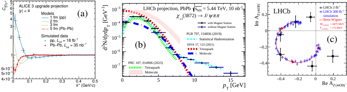
Fig. 4.10: (a) \bar{D}^0 D^{*0} correlation functions at the ALICE 3 experiment in different collision systems, where the \chi_{c1}(3872) meson is modelled as a molecular state. Figure from [128]. (b) Production of the \chi_{c1}(3872) meson in Pb–Pb collisions at the LHCb Upgrade II. Figure from [ID82]. (c) Argand diagram of the Z(4430)^- amplitude in the B^0 \rightarrow \psi(2S)\pi^- K^+ decays at the LHCb Upgrade II. Figure from [159].
