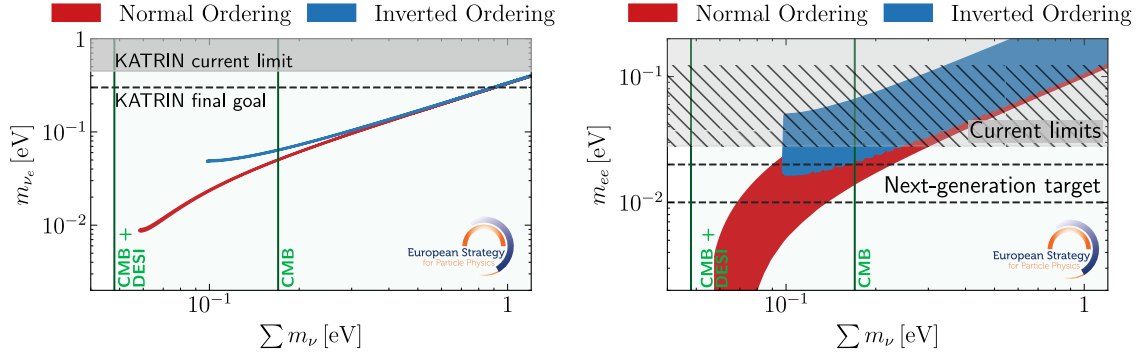
Fig. 6.1: Left: Allowed regions in the m_{\nu_e} \equiv \sqrt{\sum_i |U_{ei}|^2 m_{\nu_i}^2} versus \sum_i m_{\nu_i} plane for normal (red) or inverted (blue) orderings in the three-neutrino model. The current experimental limits on both parameters from KATRIN and cosmological measurements are shown. Right: same for m_{ee} \equiv \sum_i U_{ei}^2 m_{\nu_i} versus \sum_i m_{\nu_i} .
