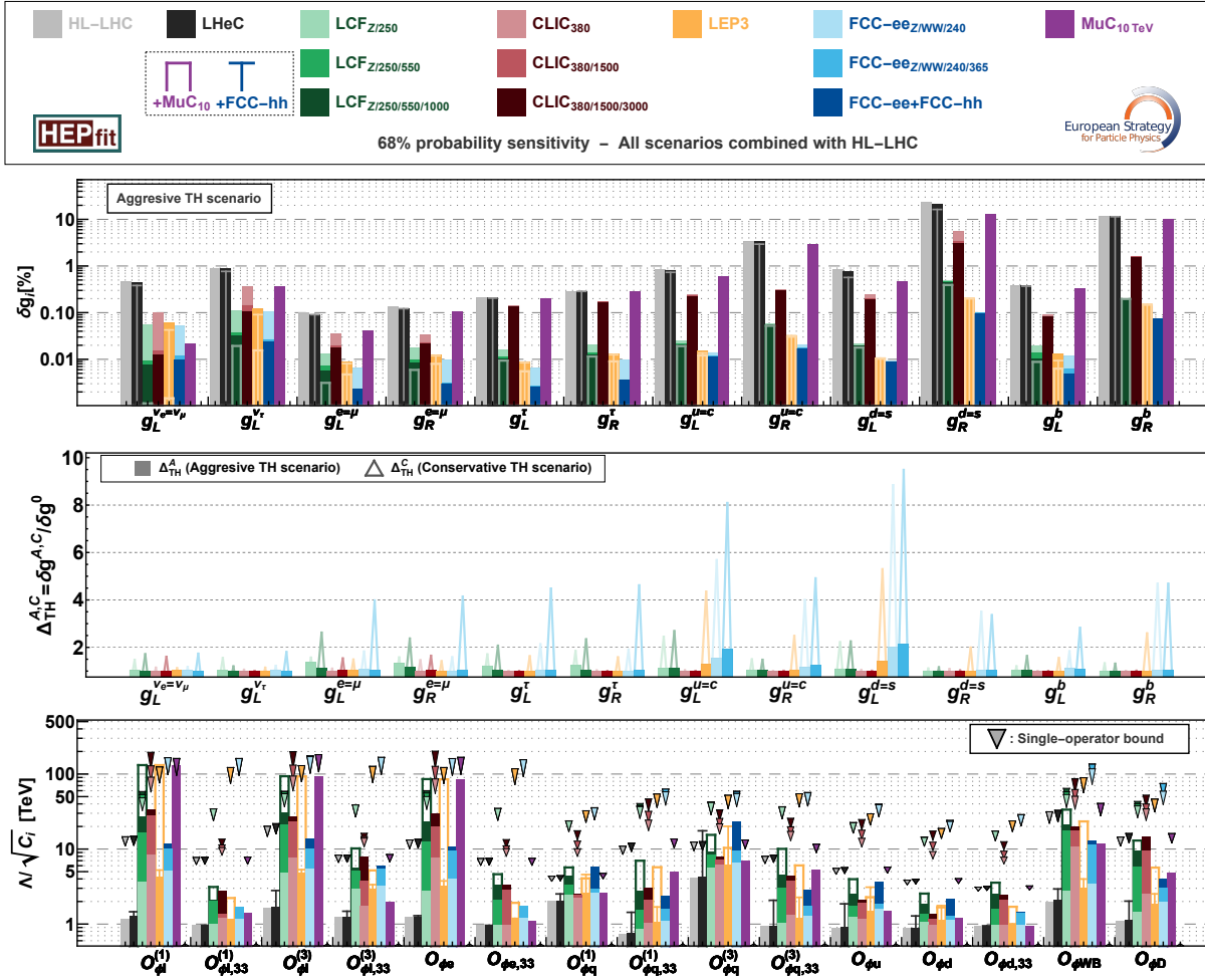
Fig. 3.5: (Top panel) 68% probability sensitivity to the combinations of operators modifying the EW couplings in the dimension-six U(2)^5 -symmetric SMEFT framework. (Middle panel) Differences in the bounds obtained using the aggressive (bars) and conservative (triangles) theory scenarios. (Bottom panel) 68% probability reach to the interaction scale associated with operators modifying each EW fermion coupling. The last two operators induce fermion-universal effects in EWPOs. The inverted triangles in this panel indicate the single operator limits for each collider. In the top and bottom panels, the empty boxes and "T" bars indicate the results from a combination of some of the colliders with the 10 TeV muon collider and FCC-hh, respectively. See text for details.
