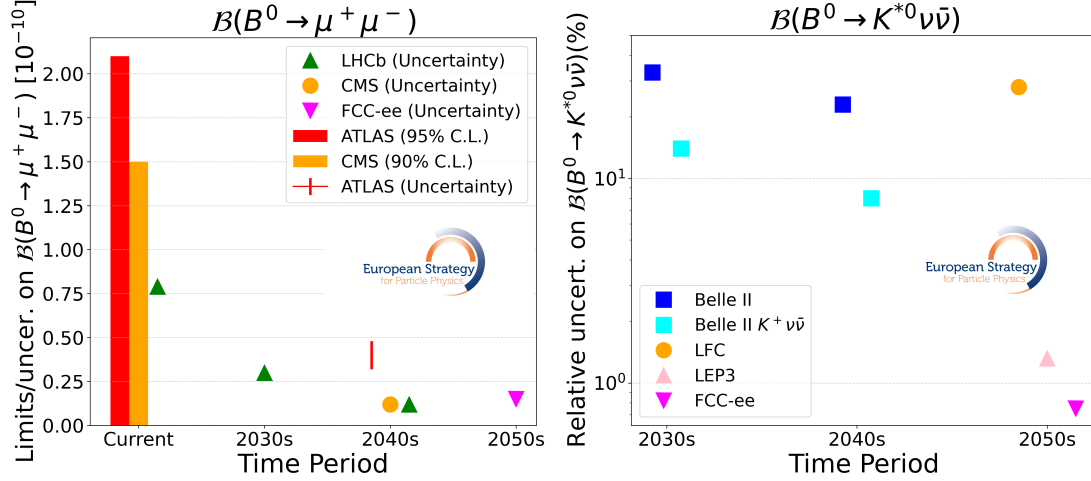
Fig. 5.14: Left: current and expected uncertainty on \mathcal{B}(B^0 \rightarrow \mu^+ \mu^-) , for different experiments [ID223, ID196]. Right: expected relative uncertainty on \mathcal{B}(B^0 \rightarrow K^{*0} \nu \bar{\nu}) .
