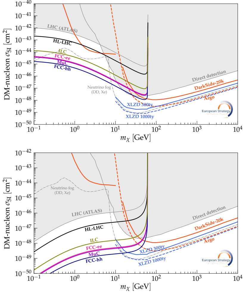
Fig. 9.9: Collider limits overlaid onto direct detection. (Top) Assuming Higgs portal scalar DM, (Bottom) Assuming Higgs portal Majorana DM. The grey area represents current constraints from direct detection experiments. Future projections for XLZD [713] and DarkSide [718] are overlaid. The notebook to generate the figure is available at [660].
