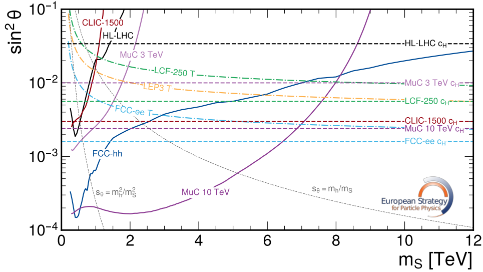
Fig. 8.7: Direct and indirect limits on a singlet scalar mixing with the Higgs boson as a function of singlet mass m_S and squared mixing angle \sin^2 \theta in the “custodial limit” BR(S \rightarrow hh) = BR(S \rightarrow ZZ) = BR(S \rightarrow WW)/2 . Solid curves indicate direct search limits, dot-dashed curves indicate indirect limits on the T -parameter, and dashed horizontal lines indicate indirect limits on the universal shift to all Higgs couplings ( c_H ), at 95% CL. Dotted grey curves indicate two characteristic scalings of the mixing angle as a function of the singlet mass corresponding to an independent singlet vacuum expectation value and an EWSB-induced singlet vacuum expectation value, respectively.
