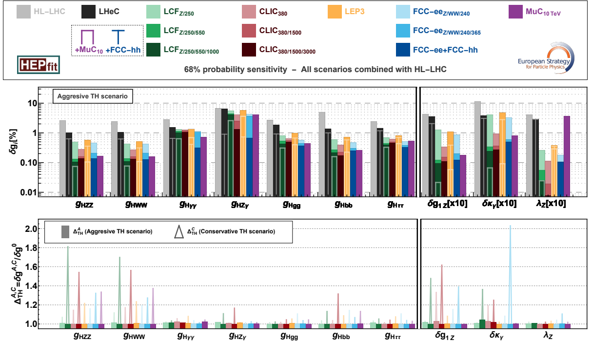
Fig. 3.6: (Top panel) 68% probability sensitivity to modifications of the effective Higgs couplings and aTGCs in the dimension-six U(2)^5 -symmetric SMEFT framework. In this panel, the empty boxes and "T" bars indicate the results from a combination of some of the colliders with the 10 TeV muon collider and FCC-hh, respectively. (Bottom panel) Impact in the fit when using the aggressive (bars) and conservative (triangles) theory scenarios.
