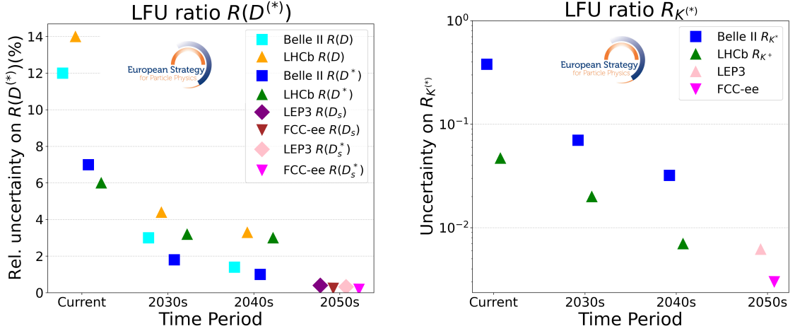
Fig. 5.13: Current and expected relative uncertainty on the LFU ratios (left) R(D^{*}) and R(D) , and (right) R_{K^{*0}} and R_{K^{+}} , in the 1.1 < q^2 < 6 \text{ GeV}^2 range, for different experiments.
