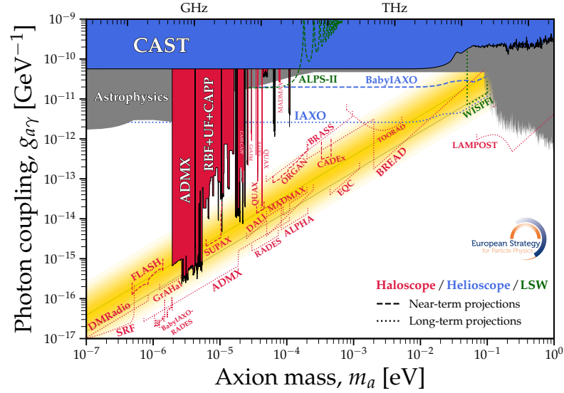
Fig. 9.2: Experimental prospects and current bounds on the coupling of axions and ALPs to photons in the sub-eV mass-scale for different types of axion searches [523]. Solid lines indicate existing experimental (red: haloscopes, blue: helioscopes, green: pure laboratory searches) and observational (grey) bounds, dashed and dotted lines for near-term and long-term prospects. The yellow shaded region indicates the typical prediction of QCD axion models. Couplings to particles other than photons can be found in [523].
