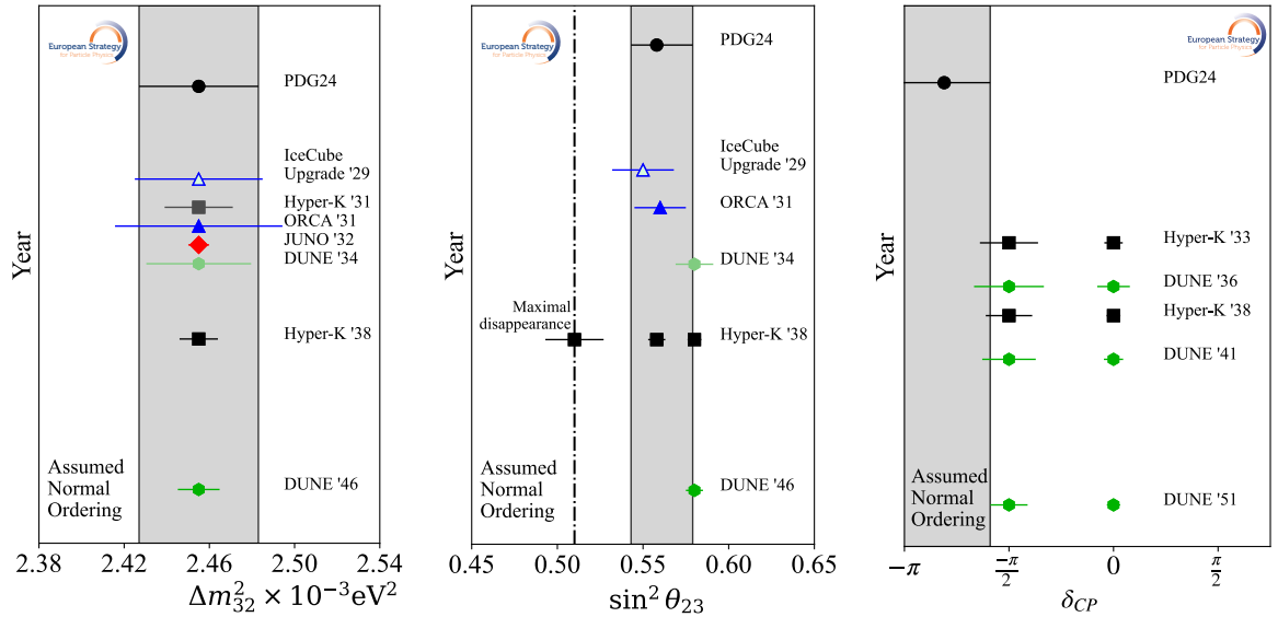
Fig. 6.4: Precision achievable by the various neutrino oscillation experiments on |\Delta m_{32}^2| , \sin^2 \theta_{23} , \delta_{CP} (from left to right). The grey area indicates the present precision (from PDG2024). The precision achievable on \sin^2 \theta_{23} depends on its value (as reported for Hyper-K, for example). For this parameter, the central point of the 3σ region is shown as the central value, and 1/6th of the 3σ range is shown as uncertainty.
