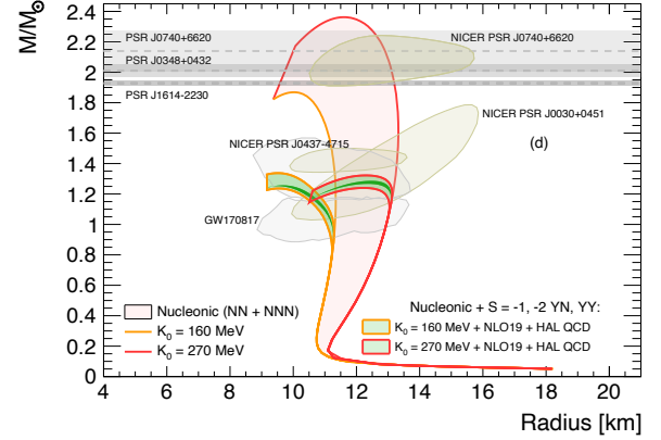
Fig. 4.8: Masses and radii of NS for a pure nucleonic EoS (red shaded area) and with the inclusion of two-body YN and YY interactions (green bands). Grey regions mark available astrophysical measurements. Figure from [139].
