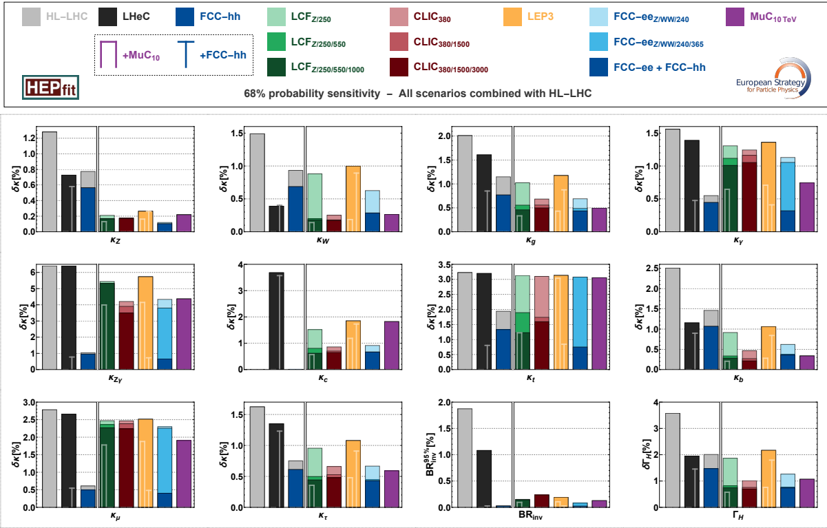
Fig. 3.1: 68% probability sensitivity to deviations from the SM on the \kappa parameters associated to the different Higgs boson couplings compared across different collider types and energies. Also shown are the 95% probability upper limits on the branching fractions of the Higgs boson into invisible (BSM) states and the precision on the indirect determination of the Higgs boson width. The pp and ep scenarios are separated from the ones of lepton colliders to indicate the difference in assumptions that go into the interpretation at the two types of colliders. In particular, the constraint \kappa_{W,Z} \leq 1 is assumed for the pp and ep interpretations. In these cases, the reported value for \kappa_{W,Z} refers to the lower bound of the 68% probability interval (i.e. 1 - \kappa_{W,Z} < \delta\kappa with 68% probability). The combinations of the LHeC and LEP3 with the FCC-hh are indicated with the "T" bars, whereas combinations of LCF and LEP3 with the 10 TeV muon collider are shown with the empty bars. For the FCC-hh only scenario, the results are shown assuming the theory uncertainties stay as in the HL-LHC (in grey) or improve by a factor of two (dark blue).
