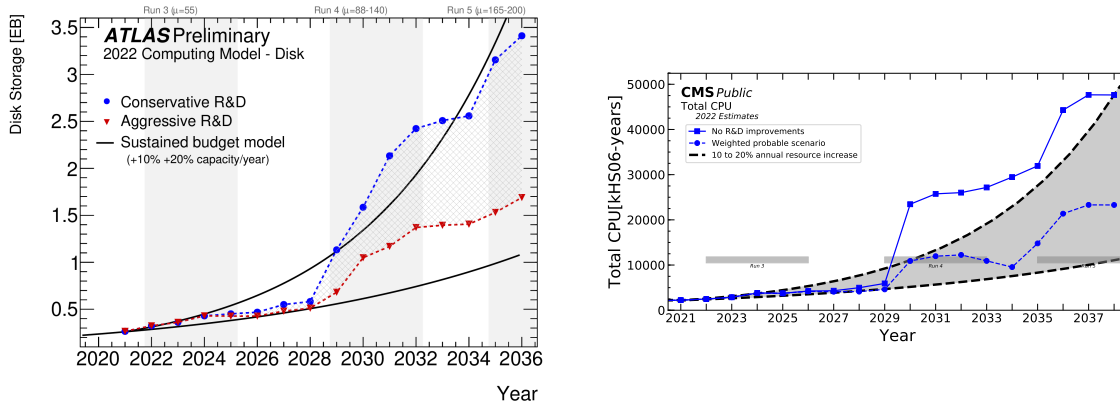
Fig. 12.1: Projected Disk needs for the ATLAS Experiment at HL-LHC, from Ref. [1068] (left). Projected CPU needs for the CMS Experiment at HL-LHC, from Ref. [1067] (right).
