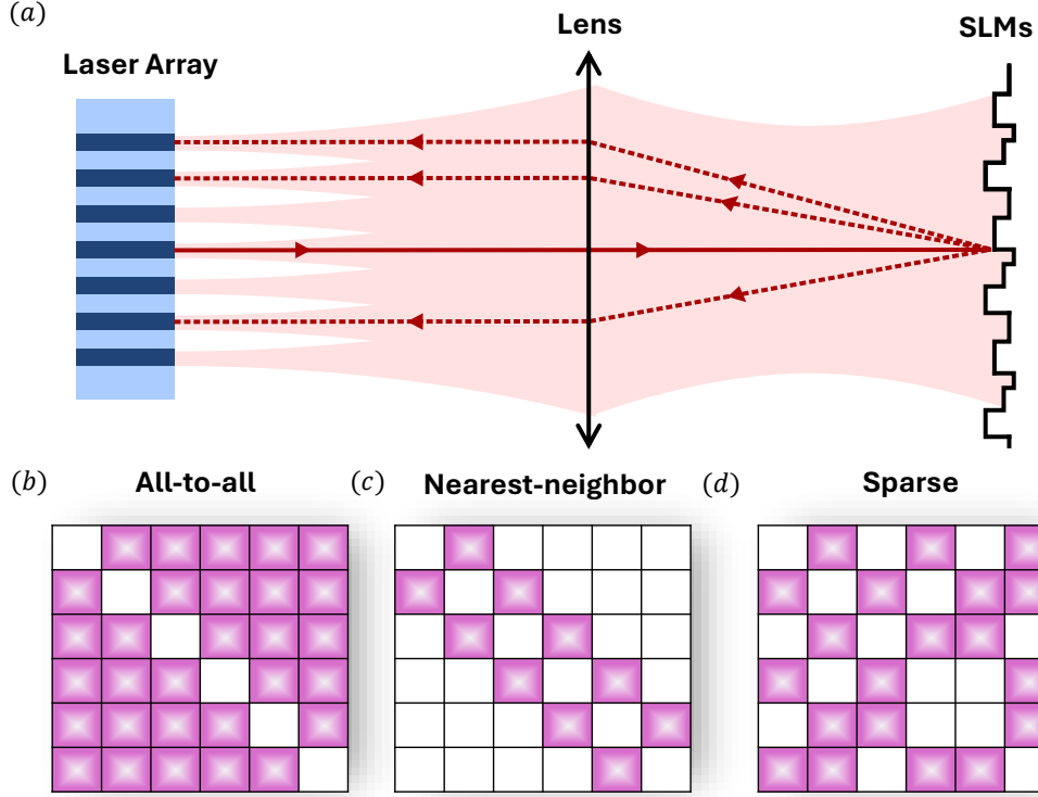
Fig. 1. Schematic diagram of laser coupling architectures. (a) Programmable laser coupling via re-programmable diffraction pattern of the SLM. (b–d) Candidate coupling structures for synchronization under frequency disorder: all-to-all, nearest-neighbor, and selectively sparse configurations, where both the horizontal and vertical axes denote the laser No., and a colored (blank) block at (i, j) indicates that lasers i and j are coupled (uncoupled).
