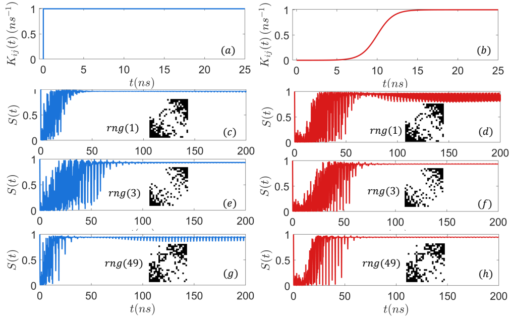
Fig. S10. Synchronization comparison between stepwise and smooth coupling ramps. Panels (a,b) illustrate two strategies for ramping the coupling strength, discontinuous (stepwise) and continuous via (K_{ij}(t) = K_{ij}/[1 + \exp[-[t - 10]]]) , with the same target coupling configuration. Panels (c–h) report synchronization outcomes for three distinct frequency-disorder realizations (labeled by rng ). Discontinuous ramps appear in (c,e,g), while continuous ramps appear in (d,f,h). In each pair (c,d), (e,f), and (g,h), the final coupling configuration after tens of nanoseconds is the same and fixed.
