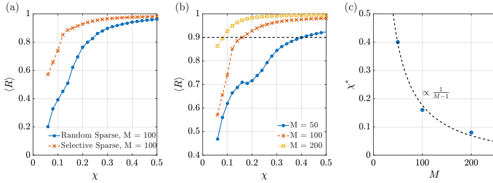
Fig. S5. Simulation results of the linear coupled network. (a) Average order parameter \langle R \rangle of the dominant super-mode \vec{v}^{m_{\max}} as a function of connectivity \chi for M = 100 lasers array. The blue dot are for a random sparse matrix and the red cross for a selective one. (b) Comparison of the average order parameter as a function of connectivity for different number of laser in a selective sparse configuration. Blue dot is for M = 50 , red cross M = 100 and yellow square for M = 200 . The dashed black line is set to \langle R \rangle = 0.9 and used to define the critical connectivity \chi^* . All results are the average of 100 normally distributed frequency realization with standard deviation of \sigma = 14 rad/ns. The Random sparse configuration is also average over 10 different random configuration. (c) Scaling of the critical connectivity \chi^* as a function of the number of laser M in the array for a selective sparse configuration.
