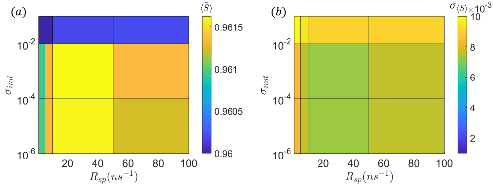
Fig. S7. Robust synchronization against dynamic and initial-condition noises. The optimal sparse laser network is from Fig. 2 in the main text, obtained from the island-based genetic algorithm. (a,b) Color-coded plot of the average synchronization strength \langle \bar{S} \rangle and the standard deviation of \langle S \rangle , respectively, in the 2D parameter plane of (R_{sp}, \sigma_{\text{init}}) , where four values are chosen for each parameter: R_{sp} = \{5, 10, 50, 100\} \text{ ns}^{-1} and \sigma_{\text{init}} = \{10^{-6}, 10^{-4}, 10^{-2}, 10^{-1}\} . For each combination of \{\sigma_{\text{init}}, R_{sp}\} , \langle S \rangle is calculated using 100 independent realizations, which are used to calculate the quantities \langle \bar{S} \rangle and \bar{\sigma}_{\langle S \rangle} .
