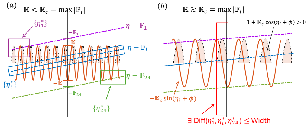
Fig. 6. Schematic of the critical effective coupling in the homogeneous all-to-all coupling. (a) Effective coupling \mathbb{K} below the critical value \mathbb{K}_c . (b) Effective coupling \mathbb{K} around the critical value \mathbb{K}_c . The rectangular regions in (a) indicate the steady-state solutions for the corresponding effective detuning \mathbb{F}_i . The red rectangular region in (b) highlights the first nearly synchronized state that emerges at the critical effective coupling, where the maximum frequency difference between lasers is about the width of the region satisfying d^2 U / d\eta^2 > 0 . The remaining notation follows Fig. 5.
