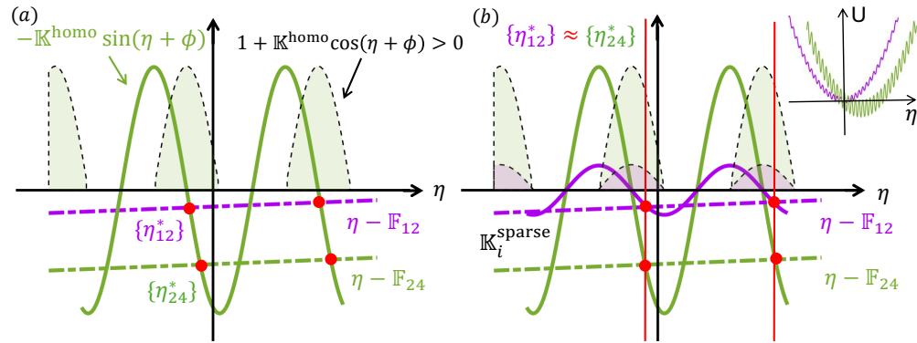
Fig. 5. Understanding synchronization in sparse networks. (a,b) Schematic illustrations of steady-state selection from the potential landscape for different lasers under homogeneous all-to-all coupling and sparse coupling, respectively. The cross intersections of Eq. (S17) are marked by the red dots in panels (a) and (b). These intersections fall within the light-shaded region that satisfies Eq. (S18). Together, they define the steady-state solutions \{\eta_{12}^*\} and \{\eta_{24}^*\} . These solutions correspond to two representative effective detuning, \mathbb{F}_{12} and \mathbb{F}_{24} associated with the 12-th and 24-th lasers, respectively. The green and purple oscillatory curves represent stronger and weaker effective coupling strengths. The inset in (b) shows the effective thermodynamic potential in (S13), consisting of a parabolic term and an oscillatory sinusoidal component. A smaller effective coupling \mathbb{K}_i^{\text{sparse}} produces a smoother potential with fewer steady-state solutions.
