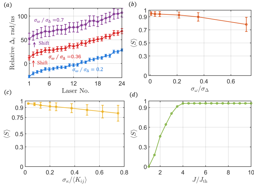
Fig. S8. Robustness in synchronization of the optimal sparse network against perturbations in frequency disorder, nodal coupling strength, and pump rate with the initial frequency standard deviation of \sigma_\Delta = 14 rad/ns. (a) Perturbation applied to the frequency detuning: \Delta_i \rightarrow \Delta_i + \delta\omega_i , where \delta\omega_i = \sigma_\omega \mathcal{N}(0, 1) , with \mathcal{N}(0, 1) denoting a standard Gaussian random variable of zero mean and unit variance. Shown is the relative frequency detuning, shifted by 40 rad/ns, for \sigma_\omega = 3, 5 and 10 rad/ns, with standard error bars calculated from 100 random realizations. (b) Resulting synchronization strength as a function of \sigma_\omega for \sigma_\omega = 0.1, 0.5, 1, 3, 5, 10 rad/ns, normalized by \sigma_\Delta . Error bars denote the standard deviation over 100 random realizations at each \sigma_\omega . (c) Synchronization strength \langle S \rangle under perturbations to the nodal coupling strength: K_{ij} \rightarrow K_{ij} + \delta K_{ij} , where \delta K_{ij} = \sigma_\kappa U(0, 1) , for \sigma_\kappa = 0.01, 0.03, 0.05, 0.08, 0.1, 0.15, 0.2, 0.25, 0.3 ns -1 . The mean coupling value is obtained by \langle K_{ij} \rangle = \sum_{ij} K_{ij} / M^2 \approx \chi^* . (d) Threshold pump rate J_{th} = \gamma_n(N_0 + \gamma/g) . The pump is scanned over J/J_{th} \in [1, 10] , and the corresponding synchronization measure \langle S \rangle is plotted as a function of J/J_{th} . In the present study, the operating pump is J_0 = 4J_{th} \approx 3.67 \times 10^8 ns -1 .
