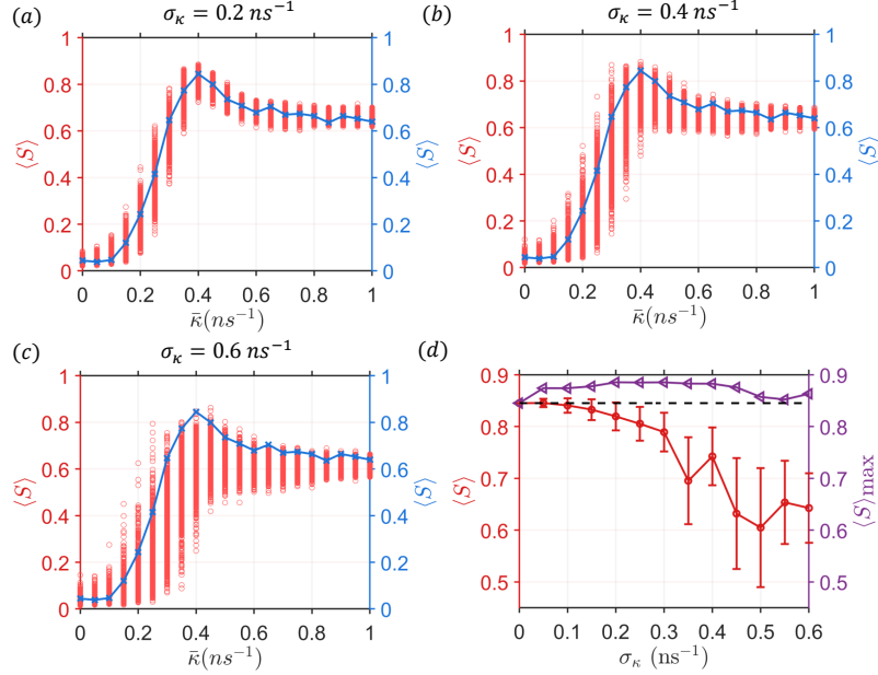
Fig. S1. Robust synchronization resonance with slightly enhanced performance in inhomogeneous all-to-all coupled diode laser networks. The nodal coupling is given by K_{ij} = [\bar{\kappa} + \sigma_\kappa \mathcal{N}(0, 1)] (1 - \delta_{ij}) with \mathcal{N}(0, 1) being a normalized Gaussian random variable. (a-c) Synchronization measure \langle S \rangle versus \bar{\kappa} for \sigma_\kappa = 0.2 \text{ ns}^{-1} , 0.4 \text{ ns}^{-1} , and 0.6 \text{ ns}^{-1} , respectively, for M = 24 , where the blue curve represents the baseline from the homogeneous all-to-all coupled network with K_{ij} = \bar{\kappa}(1 - \delta_{ij}) . The coupling strength is scanned over the range \bar{\kappa} \in [0, 1] \text{ ns}^{-1} with a step size of 0.05 \text{ ns}^{-1} . (d) Mean values and standard deviations of the randomly sampled synchronization measure \langle S \rangle at the resonance peak \bar{\kappa}^* = 0.4 \text{ ns}^{-1} versus the perturbation strength \sigma_\kappa . The corresponding peak values of \langle S \rangle_{\text{max}} as a function of \sigma_\kappa are displayed on the right. For reference, the horizontal dashed line marks the maximum \langle S \rangle obtained in homogeneous all-to-all networks, providing a baseline for comparison.
