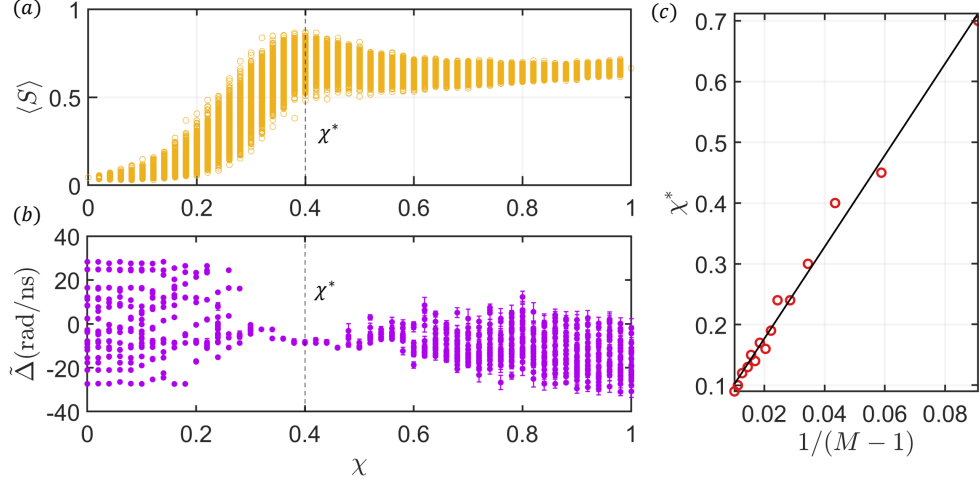
Fig. 3. Scaling behavior associated with connectivity resonance. (a) For a fixed frequency disorder with random seed rng(1) [as in Fig. 2(a)], 1000 coupling configurations are randomly generated at each connectivity \chi , and the corresponding \langle S \rangle values are shown. (b) For each \chi value in (a), the configuration yielding the highest \langle S \rangle is used to compute the final frequencies of all lasers. These frequencies are linearly fitted within moving windows of size \tau with a step size of 0.1\tau and the error bars indicate the resulting standard deviations. (c) Using the same random seed rng(1) , the scaling behavior of the optimal connectivity \chi^* is examined across different laser numbers M = [12, 18, 24, 30, 36, 42, 46, 50, 55, 60, 65, 70, 80, 90, 100] .
