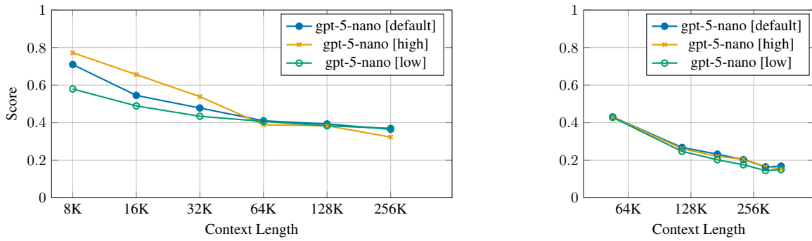
Figure 3: Comparison across reasoning levels.
