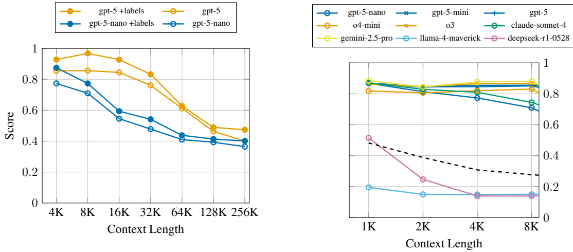
Figure 5: Comparison on OOLONG-synth: (a) we provide the gold labels in the input. This leads to a consistent but small improvement, (b) short context performance; while the top models have similar short-context performance, differences emerge as the context length grows.
