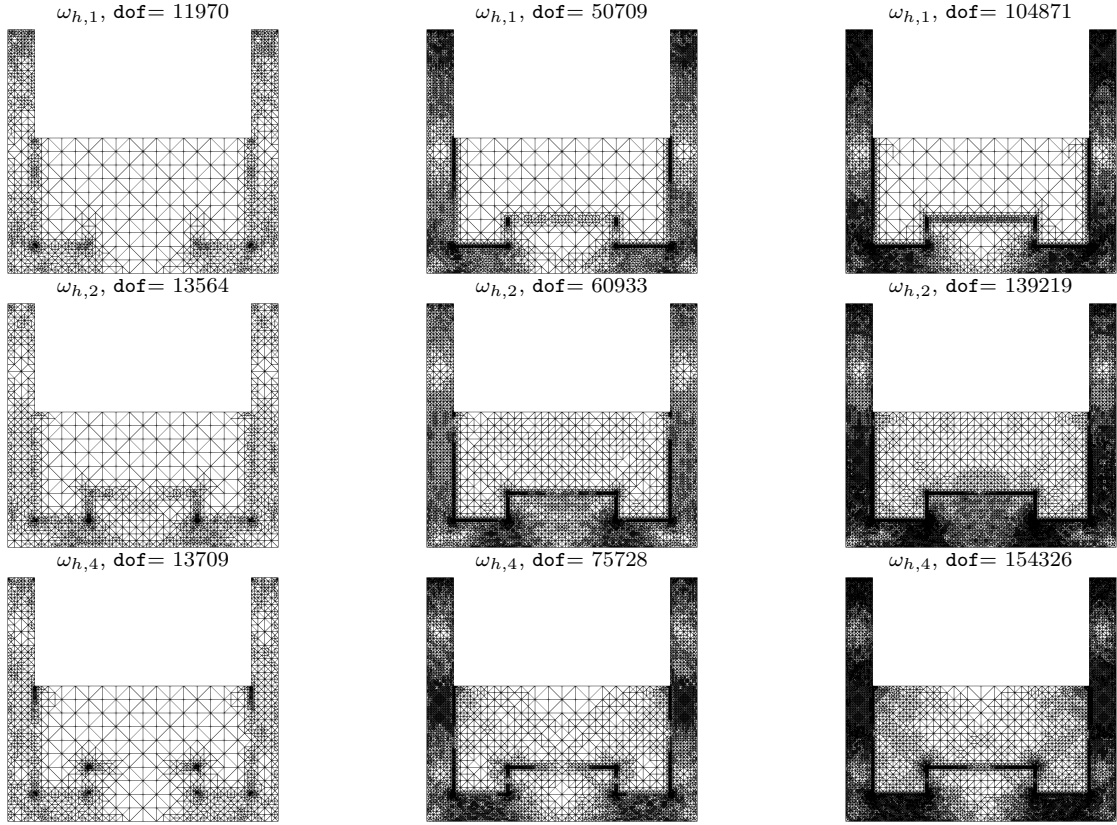
Fig. 6.5 Example 6.3. Comparison between intermediate meshes on the adaptive process for the first, second and fourth eigenfrequencies in \Omega_2 with \nu = 0.35 .
