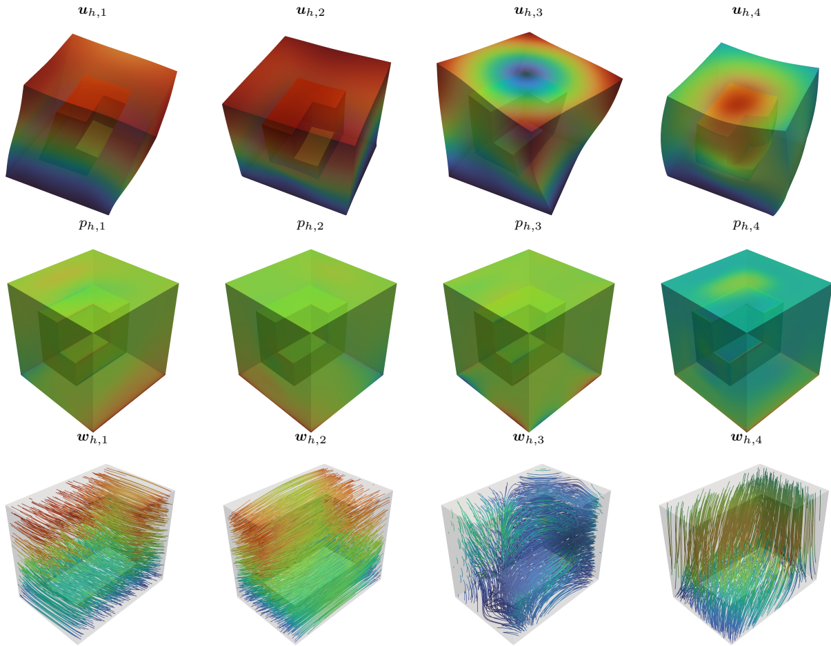
Fig. 6.9 Example 6.4. Comparison between the first fourth lowest order computed elasto-acoustic modes on \Omega_{CF} . The solid domain have been warped by a sufficiently large factor in order to observe the deformation.
