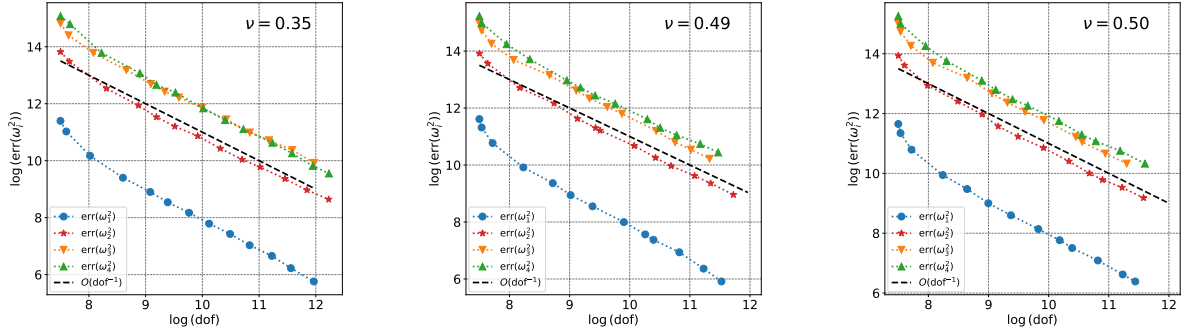
Fig. 6.6 Example 6.3. Error history for the first four lowest computed frequencies in the adaptive algorithm on \Omega_2 with different values of \nu .
