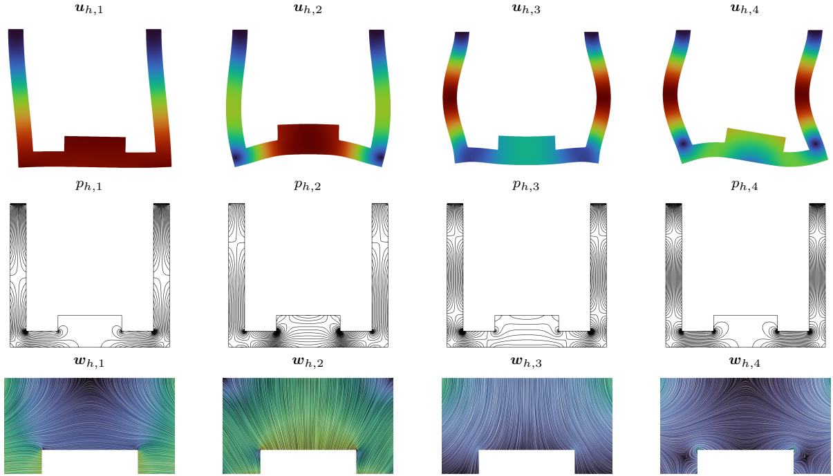
Fig. 6.2 Example 6.1. Comparison between the first fourth lowest order computed elasto-acoustic modes on \Omega_2 . The solid domain have been warped by a sufficiently large factor in order to observe the deformation.
