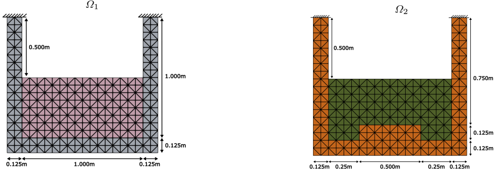
Fig. 6.1 Test 6.1. Schematic of 2D computational domains indicating dimensions, boundaries, subdomains, and using a coarse mesh with N = 2 .
