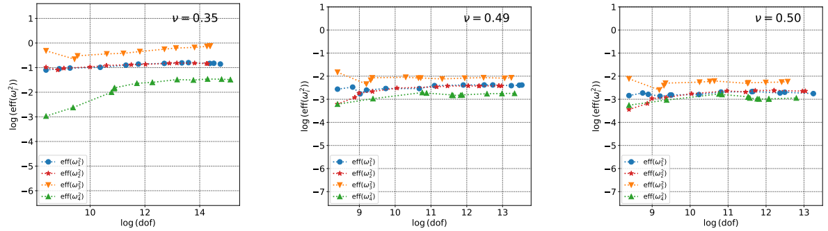
Fig. 6.12 Example 6.3. Effectivity indexes for the first four lowest computed frequencies in the adaptive algorithm on \Omega_{CF} with different values of \nu .
