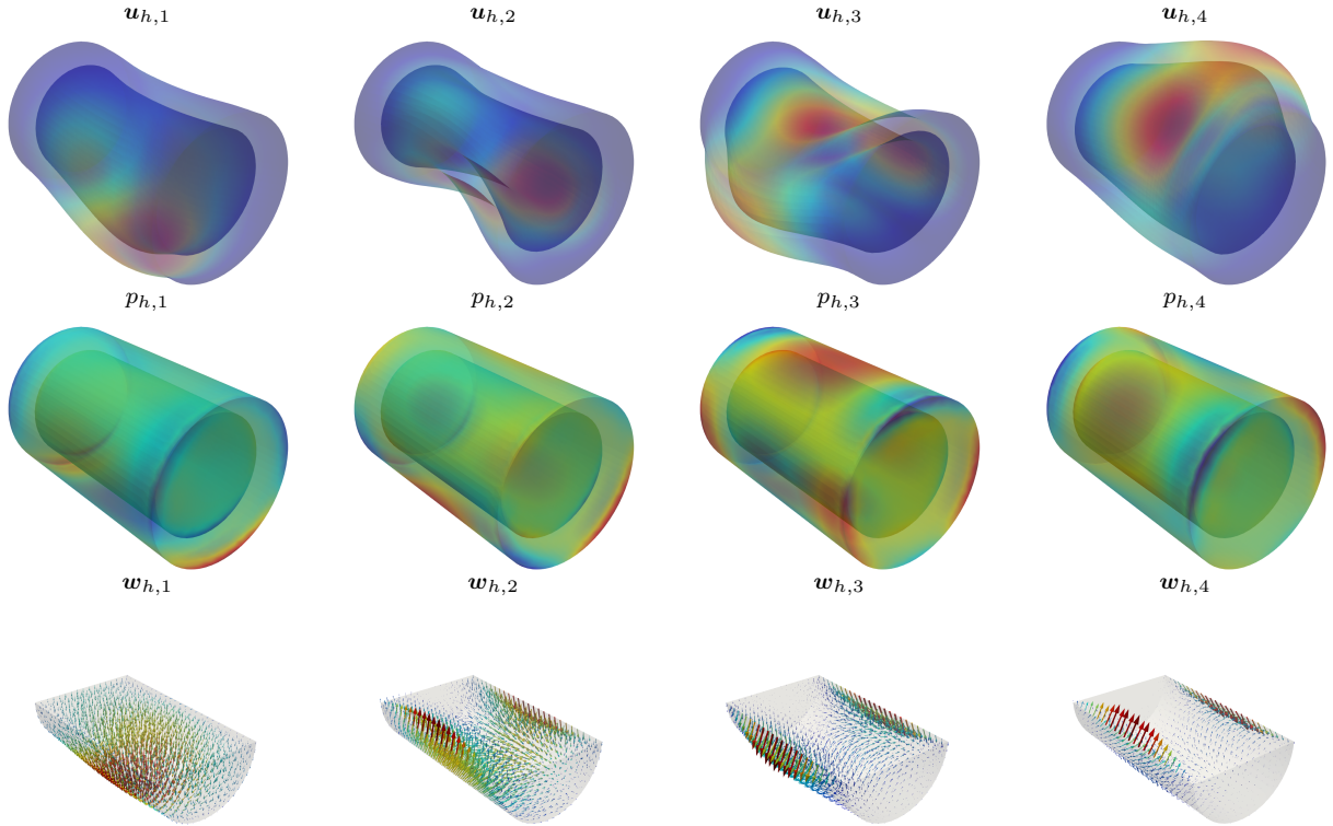
Fig. 6.4 Example 6.2. Sample numerical solutions of the first four elasto-acoustic modes on the barrel domain. The solid subdomain has been warped by a sufficiently large factor in order to observe the deformation.
