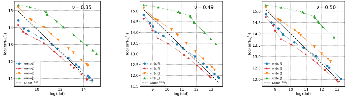
Fig. 6.11 Example 6.3. Error history for the first four lowest computed frequencies in the adaptive algorithm on \Omega_{CF} with different values of \nu .
