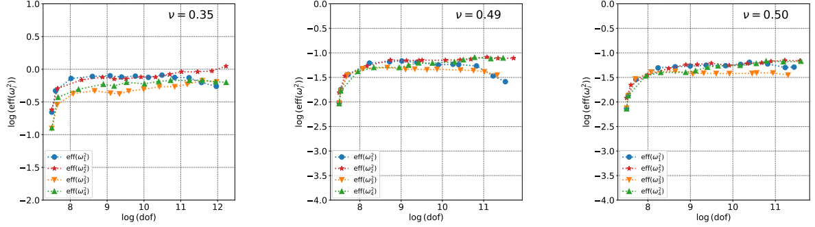
Fig. 6.7 Example 6.3. Effectivity indexes for the first four lowest computed frequencies in the adaptive algorithm on \Omega_2 with different values of \nu .
