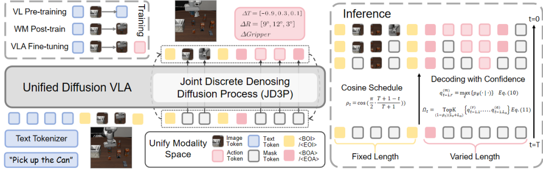
Figure 1: Overview of our Unified Diffusion VLA. We first construct a unified multimodal space by quantizing multimodal information into discrete tokens. We then formalize a Joint Discrete Denoising Diffusion Process (JD3P) to allow visual generation and action prediction to be intrinsically synergistic. Moreover, we build our model on a pre-trained VLM and conduct two-stage training. Finally, we balance performance and efficiency during inference through several key techniques.
