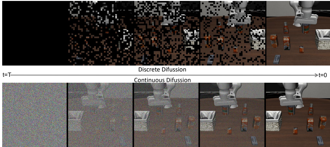
Figure 5: Qualitative Comparison of discrete diffusion and continuous diffusion.
