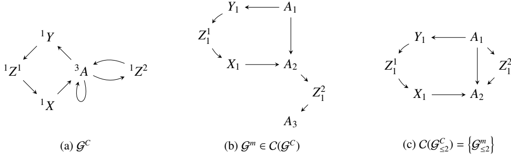
Figure 4: Figure 4a depicts a cluster \mathcal{G}^C . Figure 4b illustrates a graph compatible with \mathcal{G}^C . Figure 4c illustrates the unique graph compatible with \mathcal{G}_{<2}^C .
