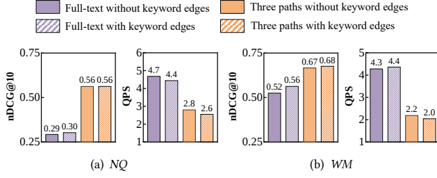
Figure 11: Performance w/o keyword edges.
