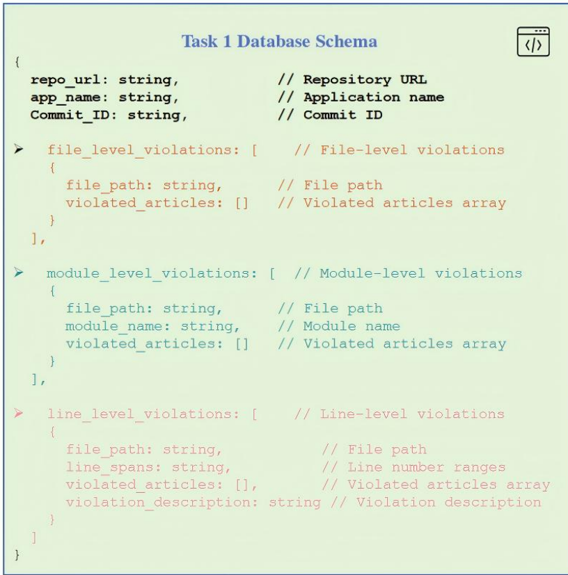
Fig. 7. The hierarchical JSON schema for task1_dataset.json . Each entry contains provenance metadata and three distinct arrays for violations at the file, module, and line levels.
