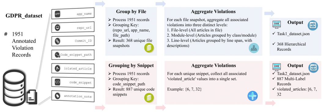
Fig. 6. The unified dataset generation pipeline. Both task-specific datasets originate from the same 1951-record source corpus. Task 1 (top branch) groups records by file, creating 368 hierarchical entries. Task 2 (bottom branch) groups records by code snippet, creating 887 multi-label entries.
