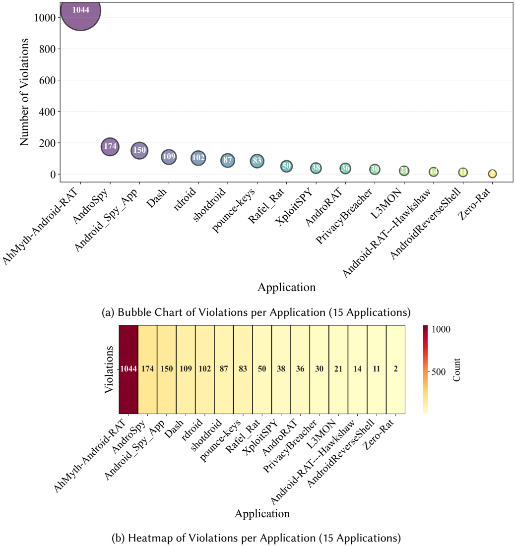
Fig. 4. GDPR violation distribution across the 15 applications in the expanded dataset. The visualizations show a heavy-tailed distribution, with AhMyth-Android-RAT contributing the majority of instances (1044).
