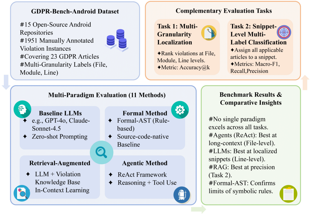
Fig. 1. A High-Level Overview of the GDPR-Bench-Android Framework.
