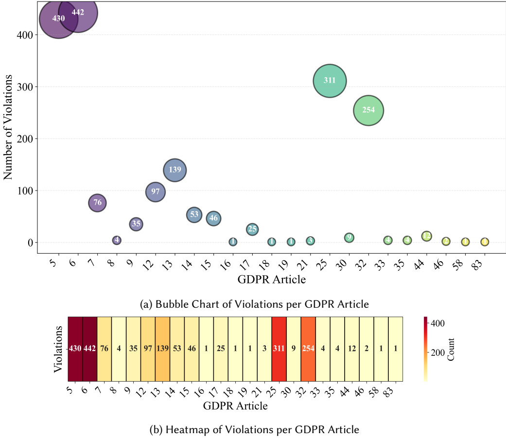
Fig. 5. Distribution of violations across all 23 GDPR articles. Articles 6 (442), 5 (430), 25 (311), and 32 (254) are the most frequent. This concentration highlights key compliance failure patterns.
