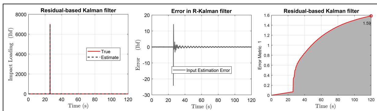
Figure 20. Structure of section “Structural loading identification in a 6-story building” in section “Discussion”: results for the 6-story shear-type building when the impact load of section “Structural loading identification in the IASC-ASCE structural health monitoring benchmark problem” is examined with the residual-based Kalman filter. True and estimated loading (first plot), error compared to true loading (middle plot), and accumulated error of Equation (25) (last plot).
