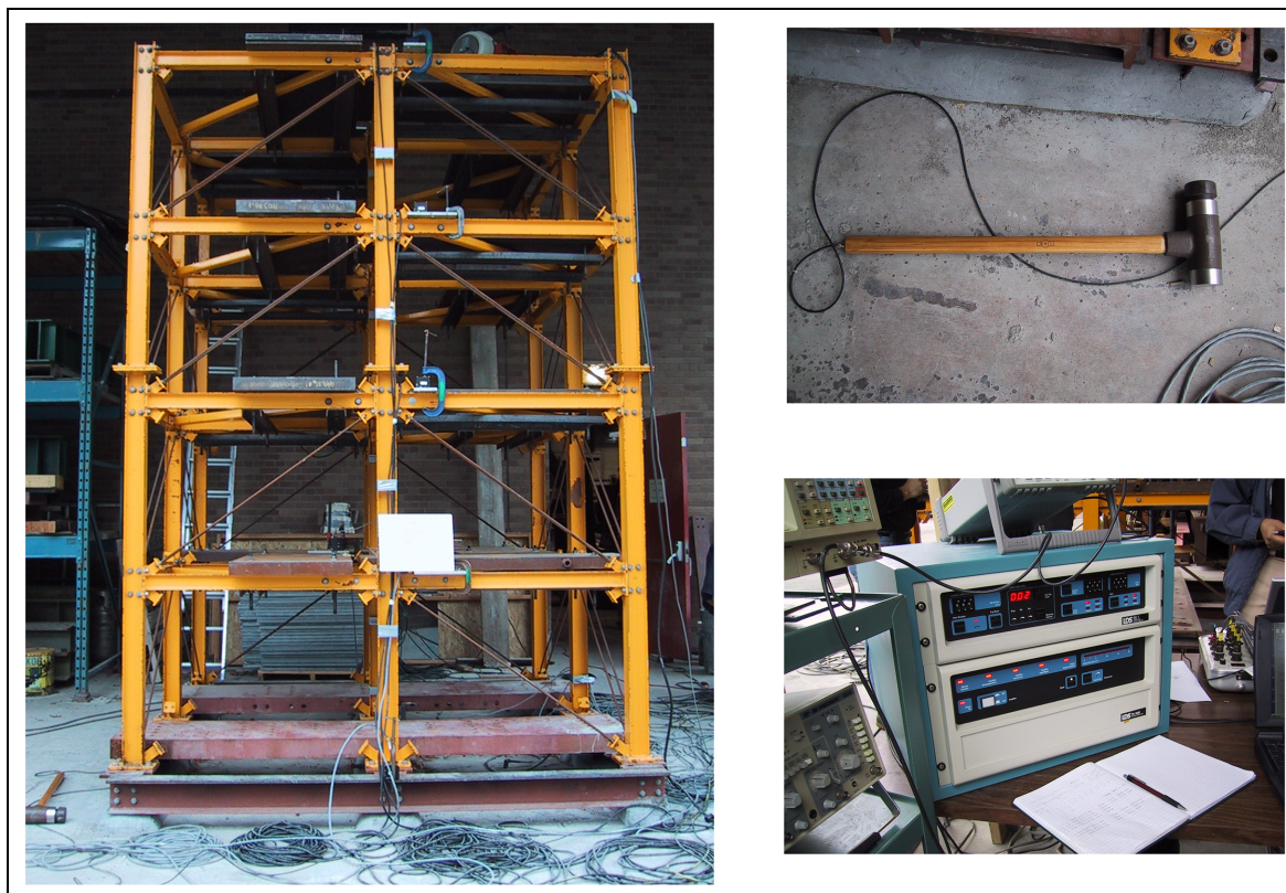
Figure 12. IASC-ASCE structural health monitoring benchmark building of section “Structural loading identification in the IASC-ASCE structural health monitoring benchmark problem”, the Dynatron 5803A 12 lbf Impulse Hammer, and the monitor and console equipment. 115
