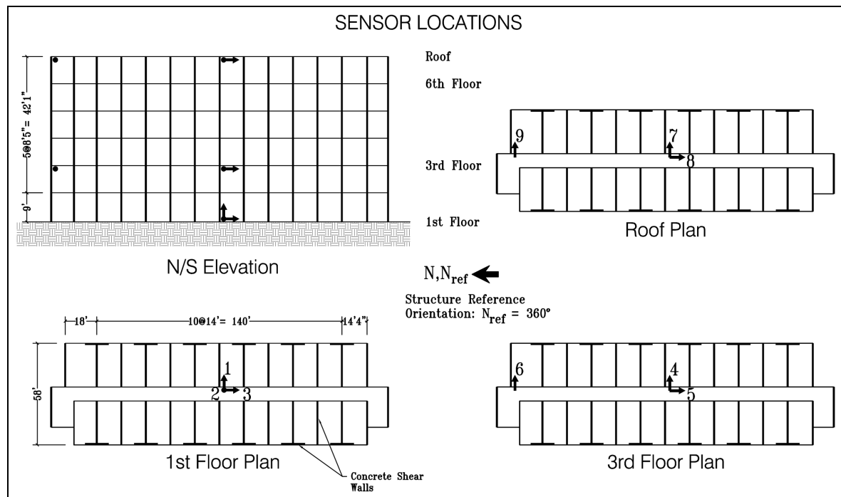
Figure 7. Sensor layout of the 6-story hotel in San Bernardino of section “Structural loading identification for a hotel in San Bernardino” (Station No. 23287).
