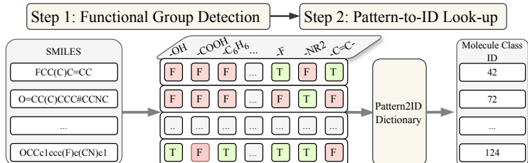
Figure 4: Overview of mapping 3D molecules to their Molecule Class IDs.
