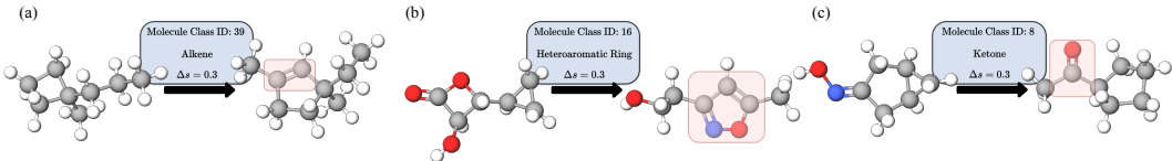
Figure 3: Visualization of molecule editing by tuning the CFG guidance scale s .
