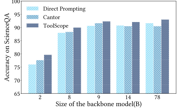
Figure 5: Scaling analysis of the size of backbone models using InternVL3 series on ScienceQA.
