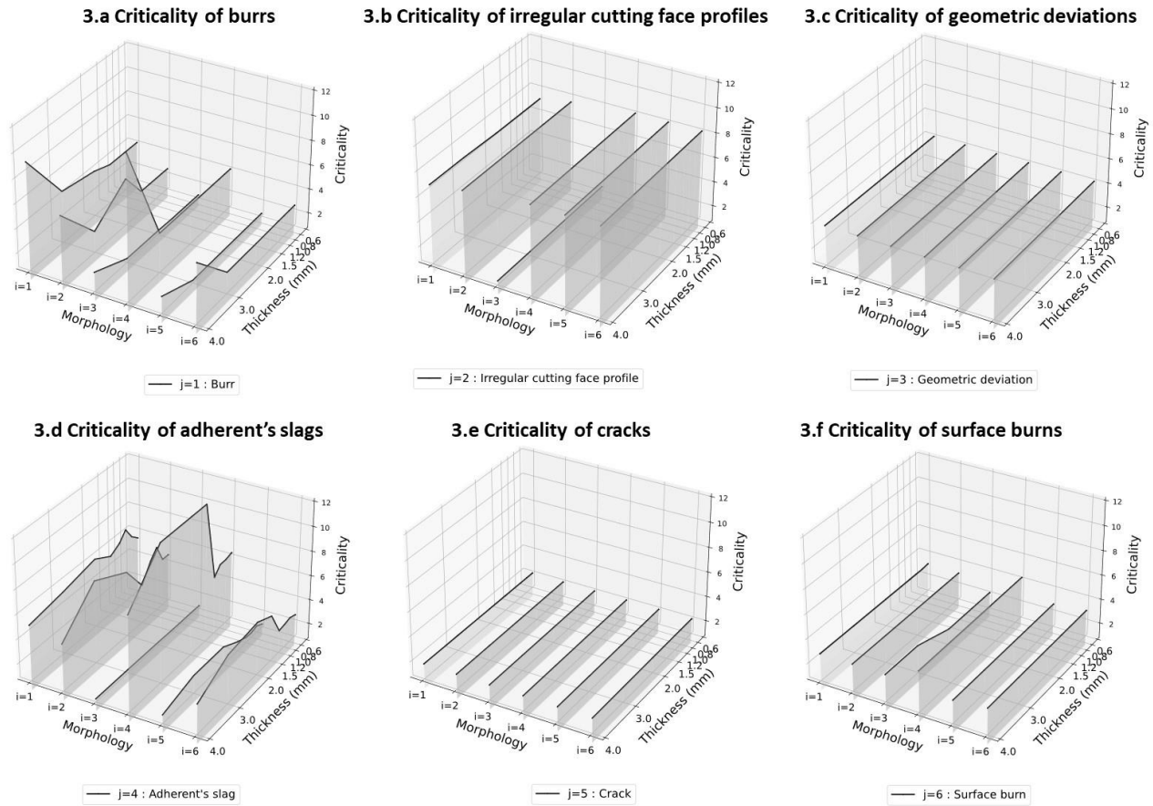
Fig. 4. Criticality of cutting defects on morphologies (Table 2) of test parts cut from DC01 steel
