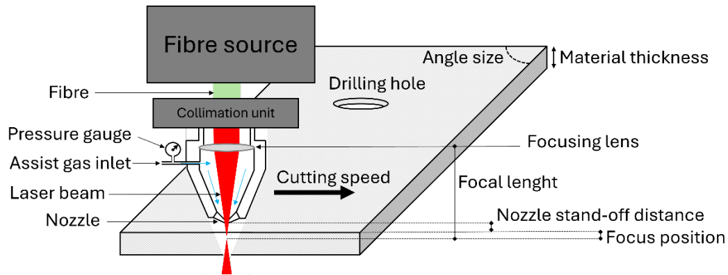
Fig. 1. Fibre laser cutting diagram
