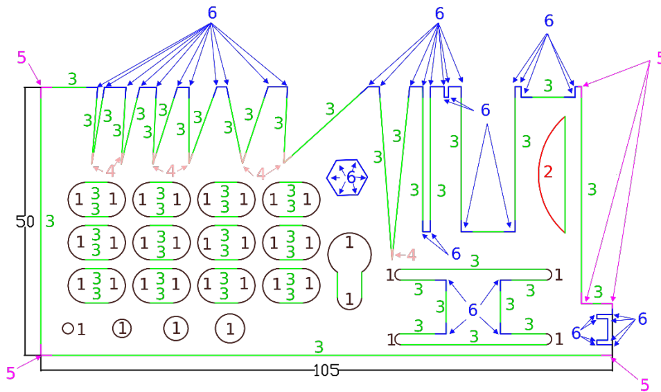
Fig. 3. Test part, with mapping of with mapping corresponding to the definition of associated morphologies (Table 2)
