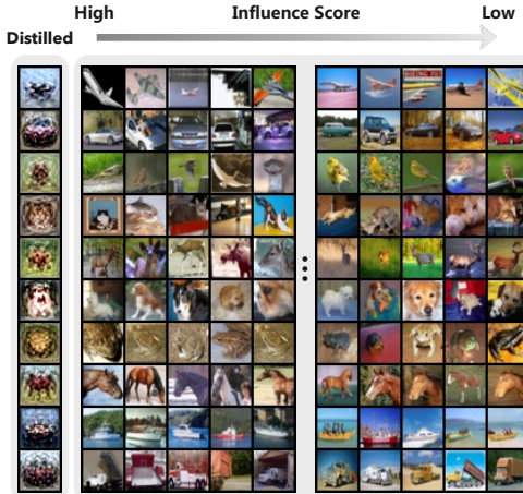
Figure 5: Synthesized images of CIFAR10 using IWD+DC.
