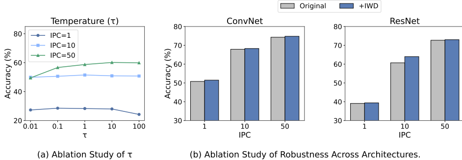
Figure 4: Ablation studies on CIFAR10. (a) Ablation Study of \tau . Effect of softmax temperature \tau under varying IPCs, showing a unimodal accuracy trend where moderate \tau achieves the best balance between emphasizing high-influence instances and retaining global information. (b) Ablation Study of Architectures. Robustness across architectures (ConvNet-3, ResNet-10), where IWD consistently outperforms corresponding baselines, demonstrating generality beyond specific backbones.
