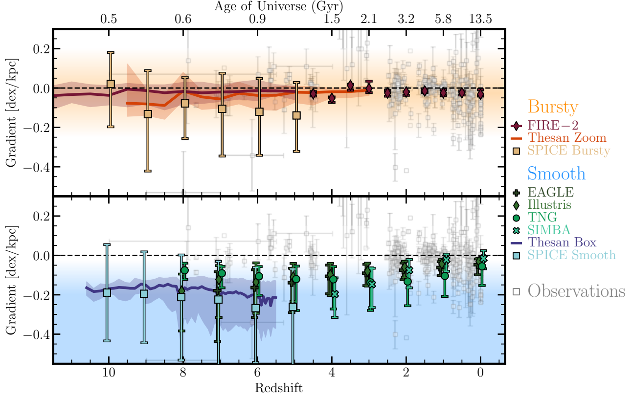
Figure 5. 13 Billion Years of Gas-Phase Metallicity Gradient Evolution in Cosmological Simulations. The composite evolution of metallicity gradients from this work and Garcia et al. (2025b) in (Top) bursty feedback models FIRE-2 (maroon diamonds), Thesan Zoom (solid orange line), and SPICE Bursty (orange squares), as well as (Bottom) smooth feedback models EAGLE (plus), Illustris (green diamonds), TNG (circles), SIMBA (Xs), Thesan Box (solid blue line), and SPICE Smooth (blue squares). The lines/markers represent the median gradient at a particular redshift while the shaded regions/error bars represent the width of the 16 – 84 th percentiles. In general, we find that bursty feedback models tend to have flatter metallicity gradients than their smooth feedback model companions, regardless of the detailed implementation of the models. The shaded regions in each panel qualitatively show where the majority of each feedback type’s gradients lie, particularly at high-redshift. We also present a compilation of observed metallicity gradients from Rupke et al. (2010b); Queyrel et al. (2012); Swinbank et al. (2012); Jones et al. (2013, 2015); Troncoso et al. (2014); Leethochawalit et al. (2016); Wang et al. (2017, 2019, 2022); Carton et al. (2018); Förster Schreiber et al. (2018); Curti et al. (2020); Grasha et al. (2022); Li et al. (2022, 2025); Arribas et al. (2024); Tripodi et al. (2024); Vallini et al. (2024); Venturi et al. (2024); Acharyya et al. (2025); Fujimoto et al. (2025); Ivey et al. (2025); Ju et al. (2025); Valé et al. (2025). Recent high-redshift observations, with the exception of those from Li et al. (2025), seem to favor more bursty feedback scenarios.
