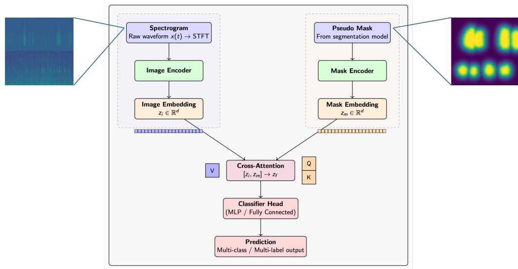
Figure 7: Architecture of the proposed model with two encoding branches and mid-fusion by cross-attention
