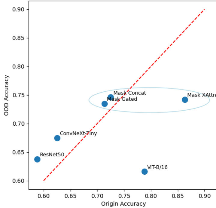
Figure 5: Comparison of the joint accuracy of the different models on the original data and on the out-of-distribution data. Models from the mask-guided methodology are highlighted in blue.
