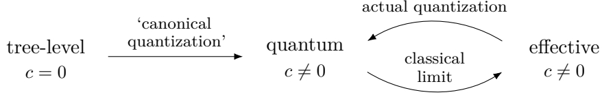
Figure 3.1: A naïve canonical quantization of the tree-level theory results in a non-zero central charge c \neq 0 . The classical limit of this quantized theory is the effective theory . It replaces the original tree-level description.
