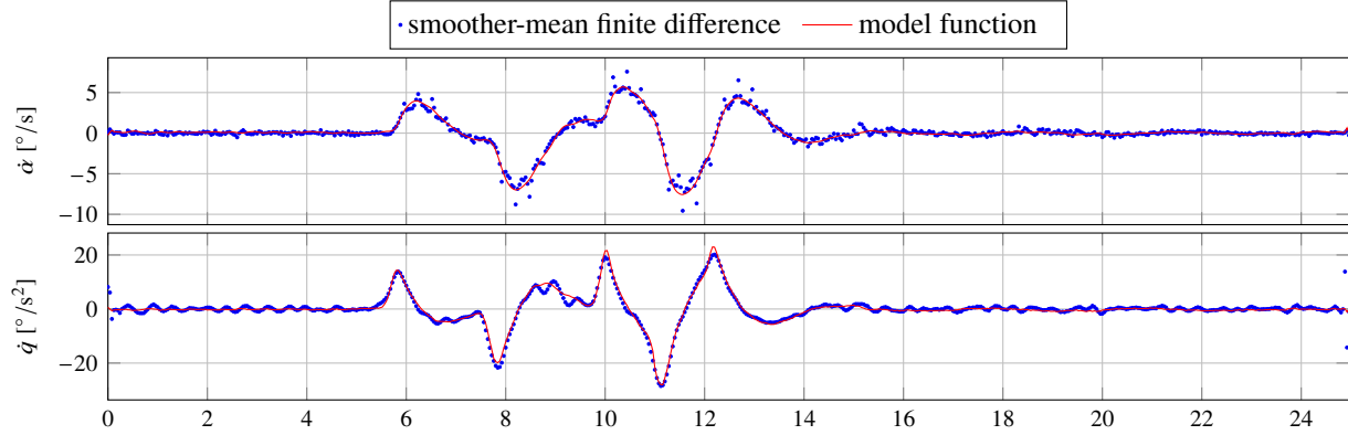
Fig. 9 Evaluation of state derivatives for the optimal parameters estimated by variational system identification on the VFW-Fokker 614 short period motion flight-test data. This is the same record that was used to estimate the model.
