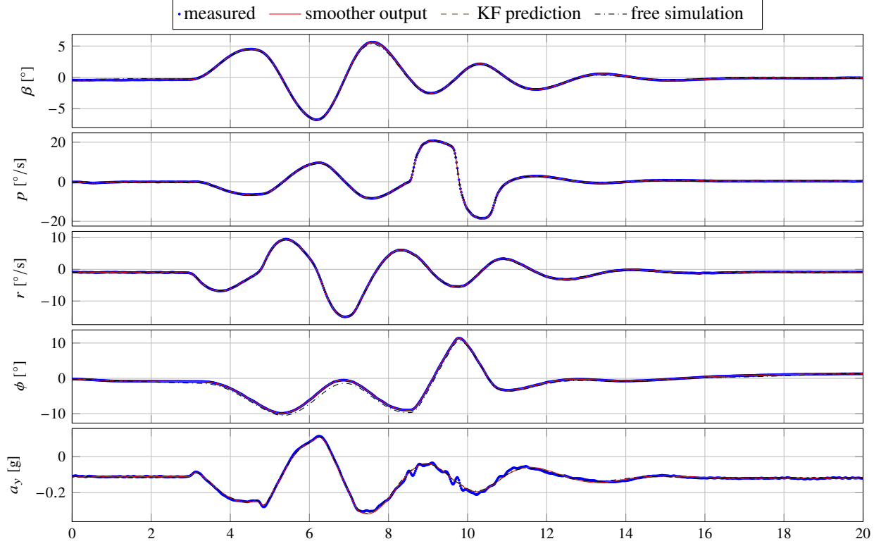
Fig. 4 Evaluation of model outputs for the optimal parameters estimated by variational system identification on the DHC-6 lateral-directional motion flight-test data. This is the same record that was used to estimate the model.
