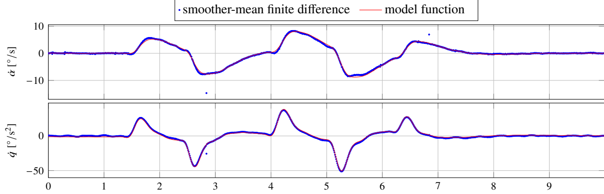
Fig. 8 Evaluation of state derivatives for the optimal parameters estimated by variational system identification on the DHC-6 short period motion flight-test data. This is the same record that was used to estimate the model.
