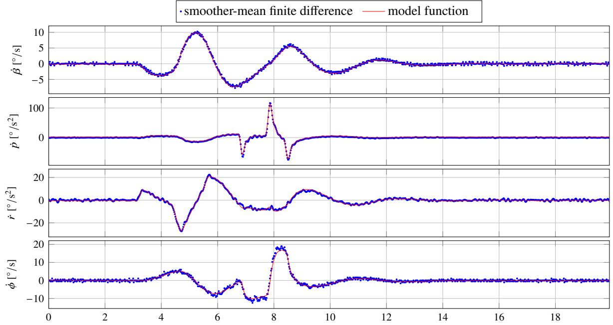
Fig. 5 Evaluation of state derivatives for the optimal parameters estimated by variational system identification on the DHC-6 lateral-directional motion validation flight-test data. This is a different record than the one used to estimate the model.
