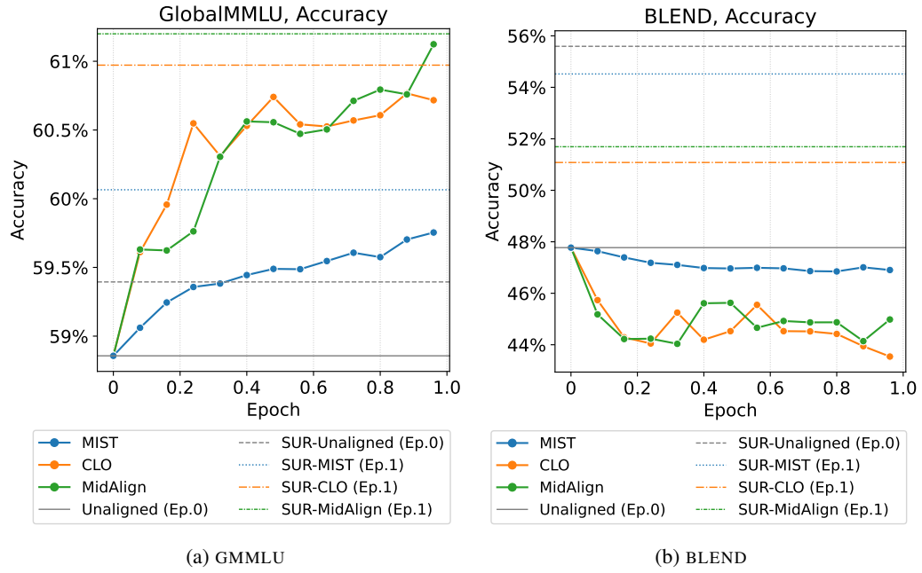
Figure 14: Learning dynamics of post-training CLA methods across alignment epochs on GMMLU and BLEND.
