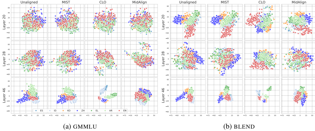
Figure 3: PCA projections of hidden representations across UNALIGNED and CLA methods. As CLA methods are applied, languages cluster more tightly, signaling stronger convergence. Yet, convergence differs by the nature of the datasets: GMMLU merges starting in the middle layers, whereas BLEND maintains separation until later stages, persisting even after CLA.
