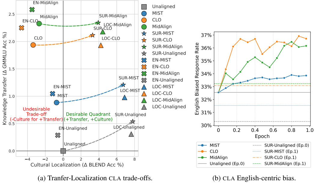
Figure 5: Left: Trade-offs between transfer and localization with steering methods. Both EN-steering and LOC-steering are applied to MIST. SUR-steering is applied on top of different post-training methods (circles), indicated by the same color or by the connecting gray dotted line. Right: Tracking English-bias of post-training CLA methods and the impact of SUR-steering on all approaches.
