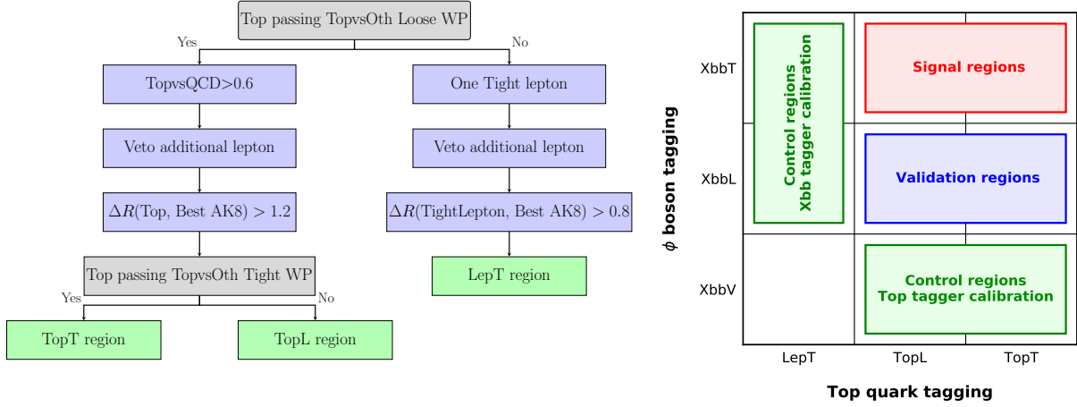
Figure 3: Left: block diagram showing the event classification based on top quark tagging. Right: schematic view of the signal, validation, and control regions defined in the analysis. The labels TopT (Top Tight) and TopL (Top Loose) refer to events where there is a top quark passing a tight working point for the TopVsOther tagger with a background rejection of 99%, or a loose working point with a background rejection of 90% while vetoing the tight working point to ensure statistical independence of the categories. The label LepT refers to events that are neither in the TopT or TopL categories, but where a top quark candidate is built via a lepton and b-jet pair. The XbbT, XbbL, and XbbV labels refer to the fact that the largest score of the XbbVsQCD tagger evaluated on AK8 jets selected in the event is in the XbbVsQCD range of ( >0.98 ), ( 0.80-0.98 ), or ( <0.80 ), respectively. Additionally, for the event to be included in the XbbV category, the mass of the jet with the largest score is required to be in the 60–220 GeV range.
