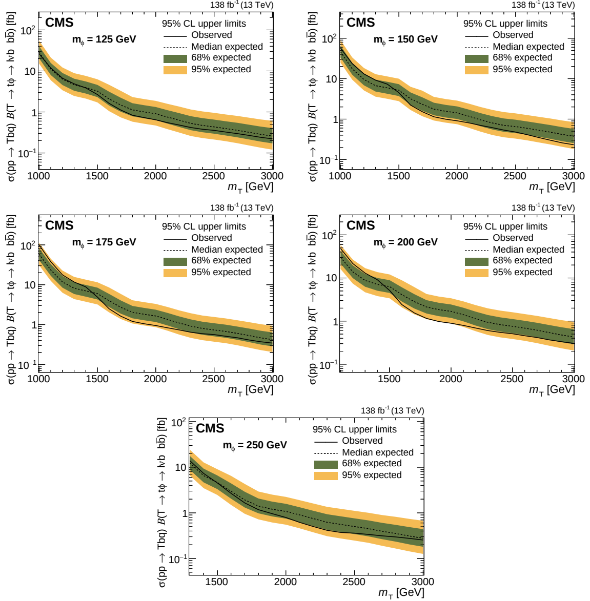
Figure 8: Observed (solid lines) and expected (dashed lines) 95% CL upper limits on the single T quark product of cross section and branching ratio for the T \rightarrow t\phi \rightarrow b\ell\nu b\bar{b}\bar{b} channel as a function of m_T , for fixed values of m_\phi , from 125 up to 250 GeV. The inner (green) and outer (yellow) bands represent the regions containing 68 and 95%, respectively, of the limit values expected under the background-only hypothesis.
