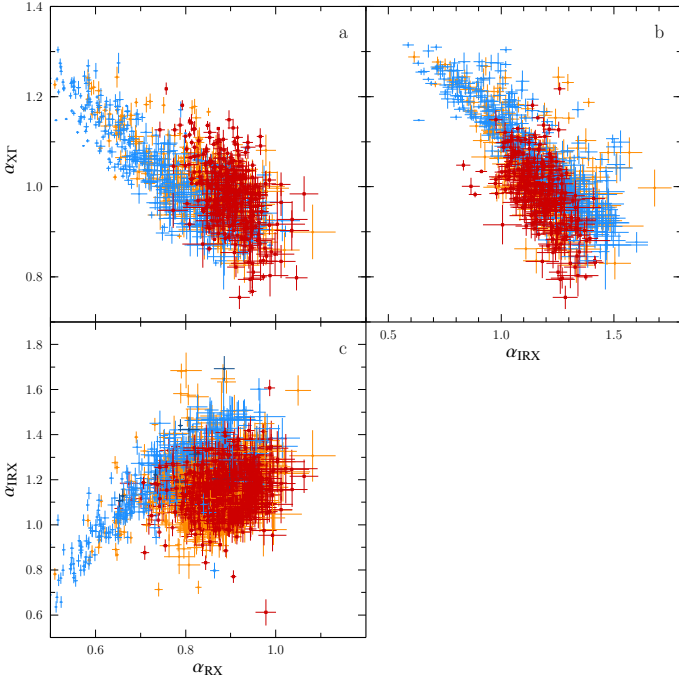
Fig. 22. Broadband spectral indices \alpha_{XF} , \alpha_{IRX} , and \alpha_{RX} against each other, following the color scheme introduced in Fig. 3. Due to the similar values obtained for \alpha_{OX} and \alpha_{IRX} , the former is not shown here.
