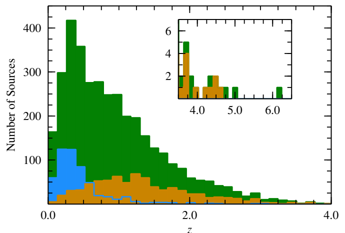
Fig. 8. Redshift distribution of BlazEr1 sources. The colors represent different sub-types. All BlazEr1 entries are shown in green (3627 sources), BLLs in blue, and FSRQs in orange. The inset shows the distribution for sources with z > 3.5 .
