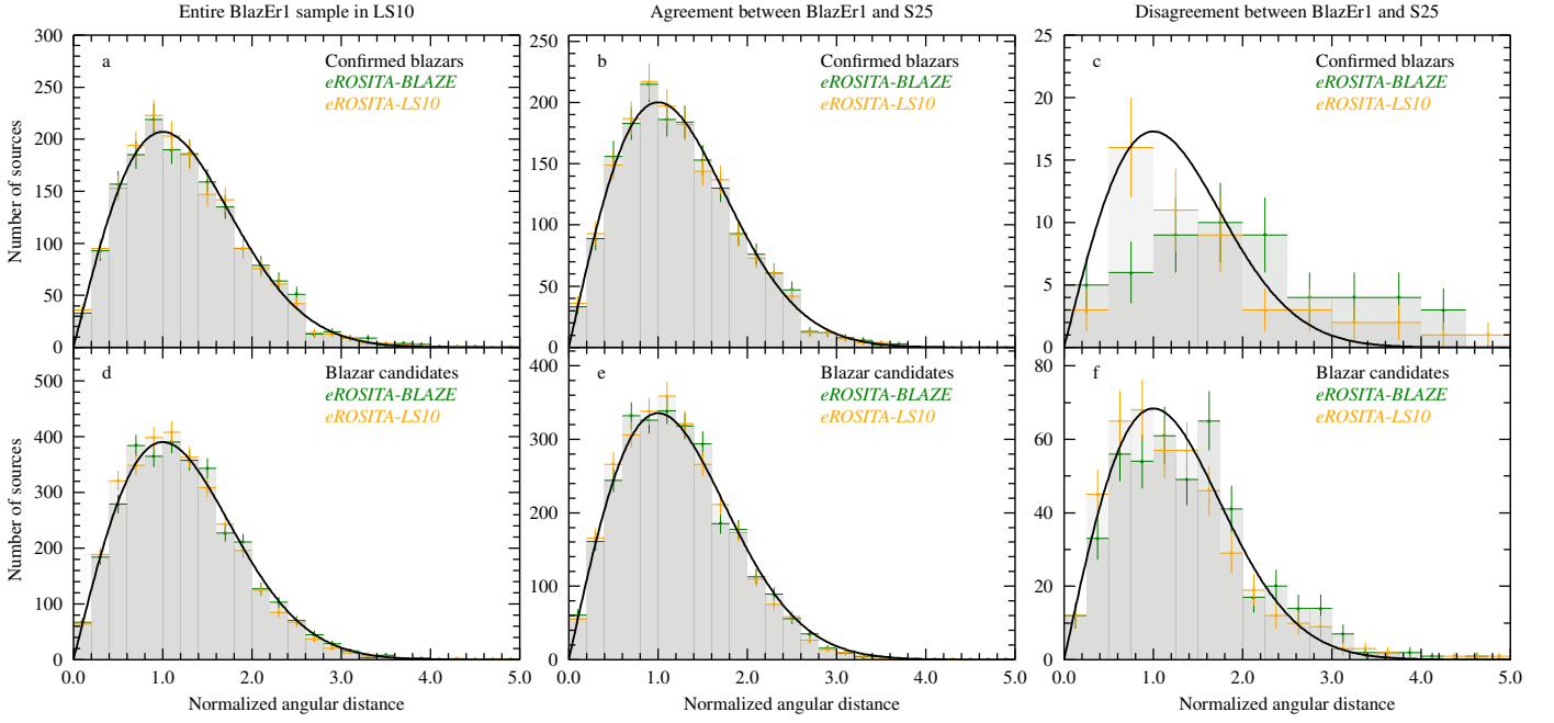
Fig. A.2. Similar to Fig. A.1, we show the separation between eROSITA and LS10 counterparts by S25 in yellow. All matches with the LS10 counterpart catalog are shown in panels a and d, whereas panels b–f only show sources where S25 provides the same or a different counterpart, respectively.
