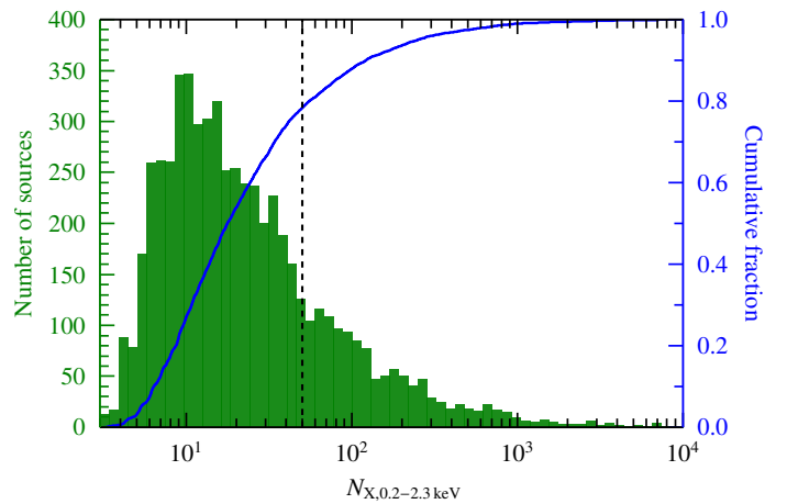
Fig. 6. Distribution of source counts with its cumulative distribution shown by the solid line curve. The dashed vertical line marks the threshold of 50 counts, above which we deem a spectral analysis meaningful. Only 20% of all sources are above this limit, while about half have fewer than 20 counts, as shown by the cumulative distribution (blue).
