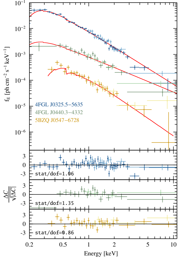
Fig. 5. Spectral fits of an absorbed power law model for three confirmed blazars with different fluxes. For 5BZQ J0547–6728, no prior X-ray observations are available. The three lower panels display the fit residuals for each source. Data from TM5 and 7 are displayed in a lighter color.
