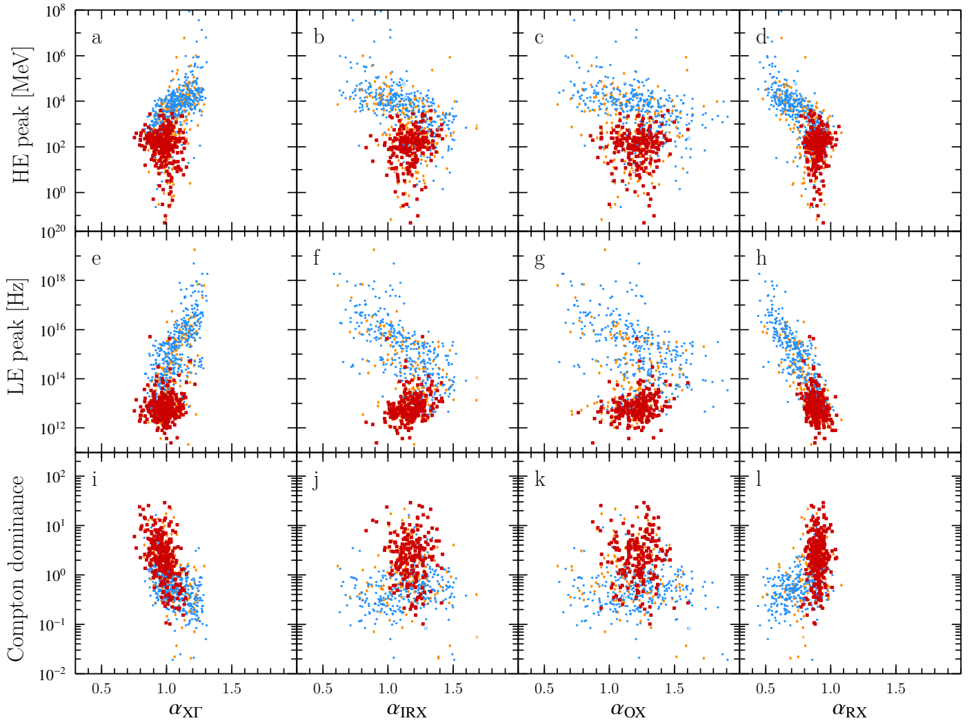
Fig. A.4. SED parameters from the 4LAC catalog as a function of various broadband spectral indices, following the color scheme introduced in Fig. 3.
