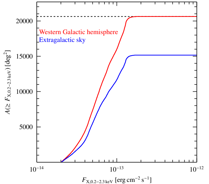
Fig. 4. Sky area in which 95% of all sources above a minimum flux will be detected with \text{DET\_LIKE}_0 \geq 10 . The dashed line indicates the total area of the western Galactic hemisphere. The red line displays the sensitivity over the entire western Galactic hemisphere, while the blue line shows the extragalactic sky excluding an area of 15^\circ below and above the Galactic plane and regions with radii of 5.5^\circ around the Large Magellanic cloud (LMC) and 3.0^\circ around the Small Magellanic cloud (SMC).
