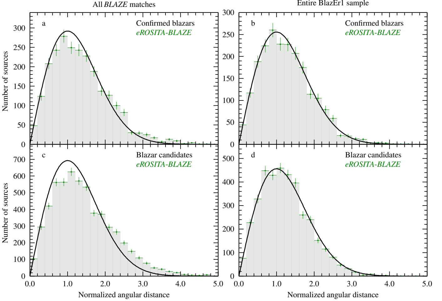
Fig. A.1. Histograms of the angular separation between the positions provided in the BLAZE catalog normalized by the respective eROSITA positional error. The upper panels display the eROSITA observed blazars and the lower panels the eROSITA observed blazar candidates. In panels a and c we show all the initial matches. In panels b and d, we show the BlazEr1 sample with applied quality and separation cuts. The theoretical Rayleigh distributions are shown as a black solid line.
