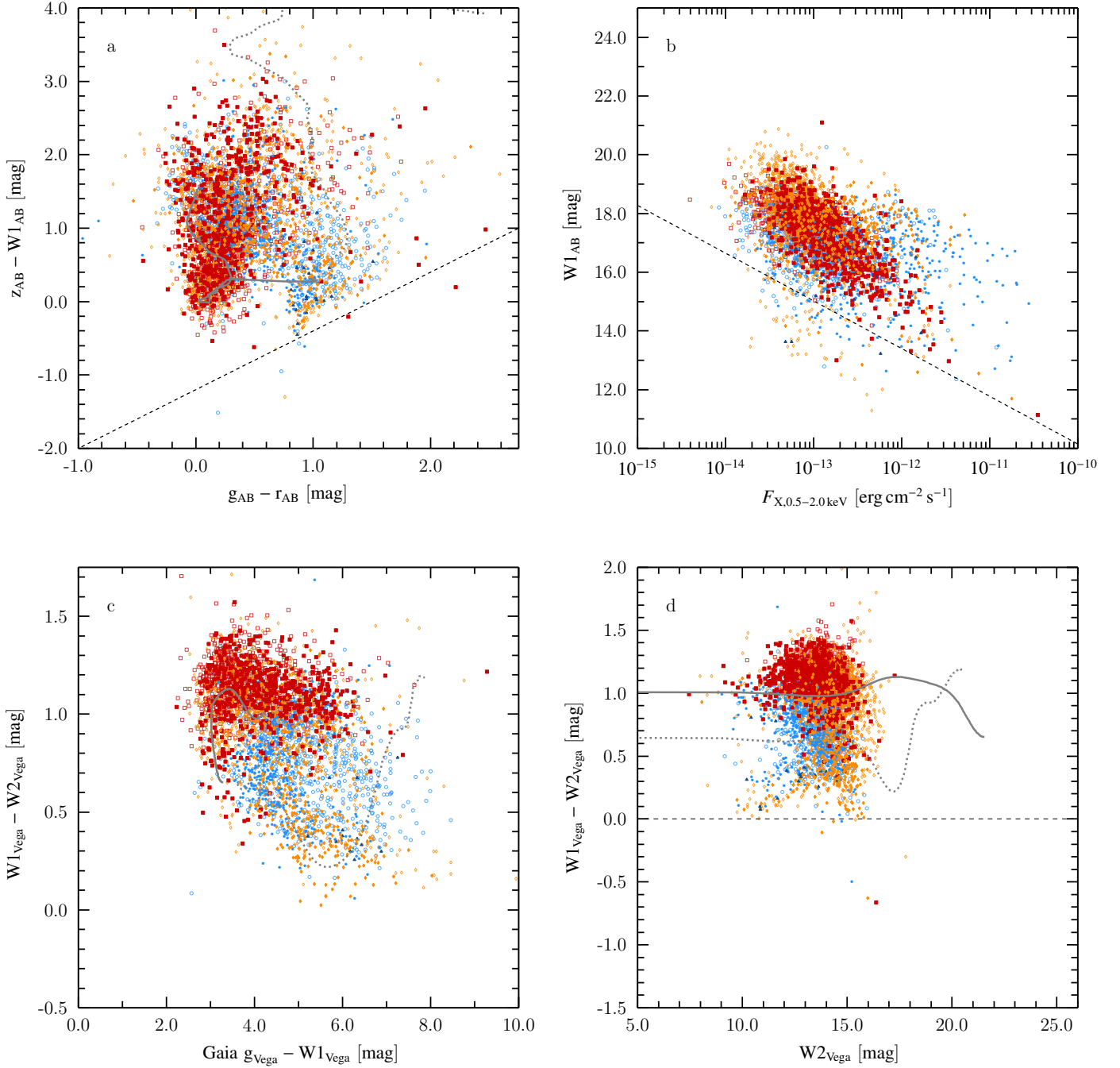
Fig. 21. Different photometric spaces combining optical, infrared and X-ray data, similar to Salvato et al. (2022; ; Fig. 18) for point sources detected in eFEDS, using the color scheme introduced in Fig. 3. Solid gray lines show positions usually occupied by quasars, whereas the gray dotted lines corresponded to Seyfert 2 galaxies. The dashed black lines in the upper panels distinguish between Galactic and extragalactic sources.
