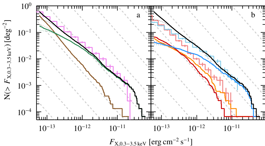
Fig. 14. \log N - \log S distributions for sources within the extragalactic sky. Panel a : comparison of the total sample of eROSITA observed blazars and blazar candidates (black) with the distribution by Giommi & Padovani (2015; purple). Green and brown show the \log N - \log S for both classes separately (green: eROSITA observed blazars, brown: observed candidates). Panel b : comparison of the predictions of Giommi & Padovani (2015) for BLLs (light blue) and FSRQs (light red) with eROSITA measurements for BLLs , FSRQs , and BCUs , using the color code of Fig. 3).
