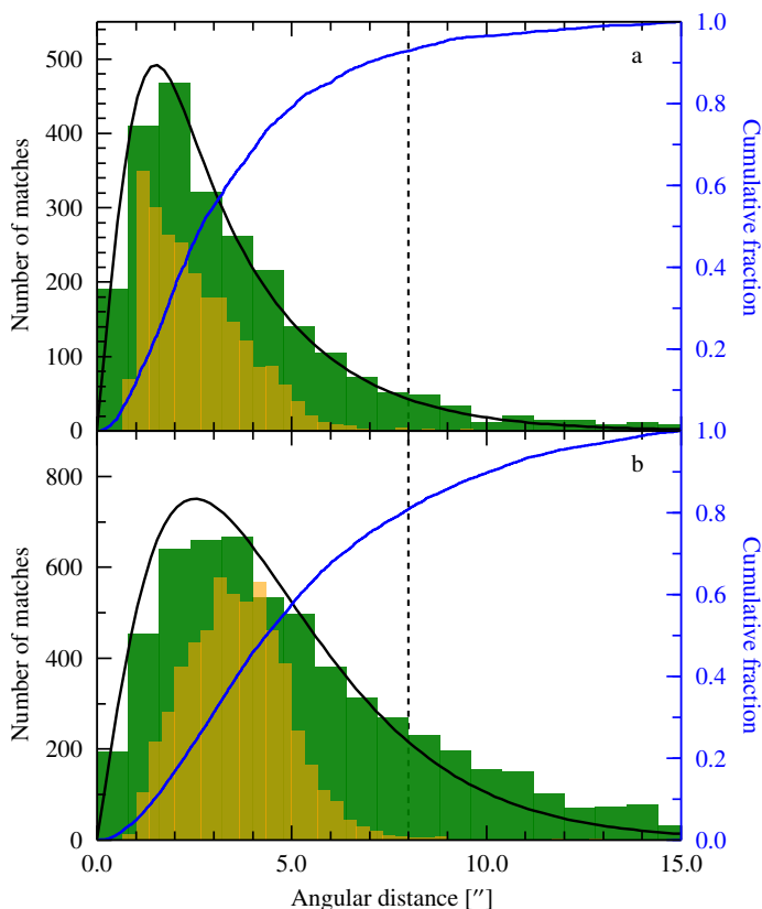
Fig. 2. Histograms of angular separation between BLAZE catalog and eROSITA positions (green) with the distribution of the matched eROSITA source positional uncertainty overlaid (yellow). The vertical line at 8'' indicates the distance threshold for the final sample. The cumulative distribution of the angular separation is shown in blue. a Sample of eROSITA observed blazars with 93% of the matches found within 8'', and 55% and 79% within 3'' and 5'', respectively. b eROSITA observed blazar candidates. Only 81% of matches are within 8'', and 31%/58% within 3''/5''. We show Rayleigh distributions (black) for illustrative purposes, calculated following Merloni et al. (2024; Eq. 3, assuming F = 0.8 ).
