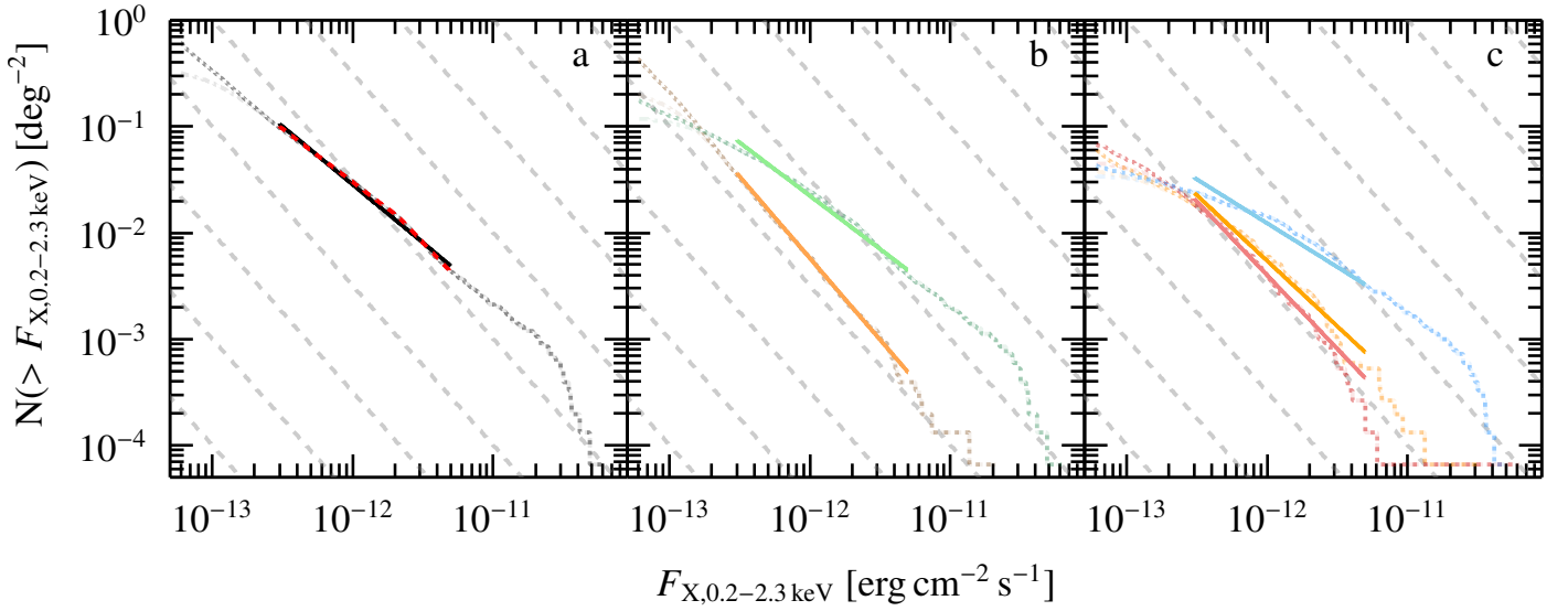
Fig. A.3. log N -log S distributions of different BlazEr1 subsamples, similar to Fig. 14 but for the eROSITA main band and including the fit results listed in Table 5. The color scheme is the same as in Fig. 14. The red line in the left panel shows the best fit broken power law for the entire sample ( \alpha_1 = 1.003 \pm 0.013 , \alpha_2 = 1.39 \pm 0.07 , F_{X,\text{break},0.2-2.3\text{ keV}} = (2.11 \pm 0.26) \times 10^{-12} \text{ erg cm}^{-2} \text{ s}^{-1} , C = 30.6 \pm 2.5 \text{ deg}^{-2} ).
