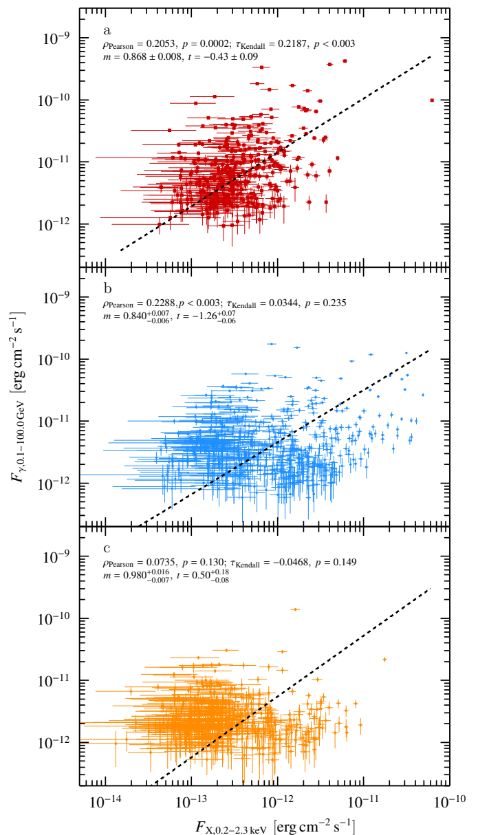
Fig. 17. Fermi -LAT fluxes (4FGL-DR4; Abdollahi et al. 2022) compared with eROSITA fluxes. The three panels show the different subtypes, following the color scheme introduced in Fig. 3 (a: FSRQs , b: BLLs , c: BCUs ). The Fermi -LAT uncertainties are scaled to match the confidence limit of the eROSITA data.
