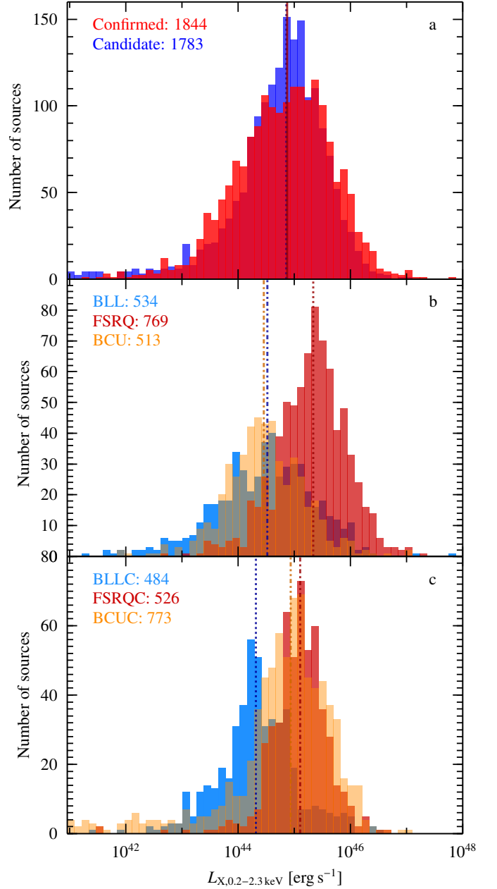
Fig. 10. Luminosity distribution for all sources with reliable redshifts. The panels show distributions for different subgroups of the eROSITA blazars and eROSITA blazar candidates, with vertical lines indicating the median luminosity for each subgroup (see Table 3).
