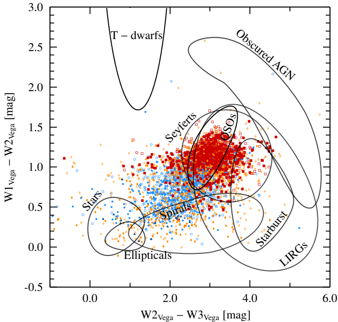
Fig. 20. WISE color-color diagram, following the color scheme introduced in Fig. 3. Regions populated by different types of AGN, as well as other objects, are shown. Compare our results to Salvato et al. (2018; Fig. 9), for a color-color diagrams of the 2RXS and XMMSL2 samples.
