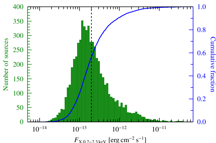
Fig. 7. Flux distribution in the BlazEr1 catalog. The majority of sources have fluxes below the survey completeness limit on the western Galactic hemisphere, the vertical line marks this limit. The cumulative distribution is shown in blue.
