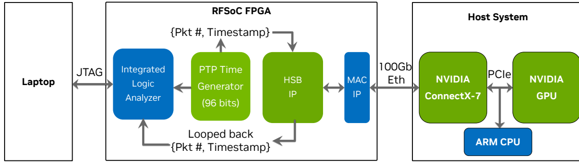
Fig. 3. Proof of Concept flow
