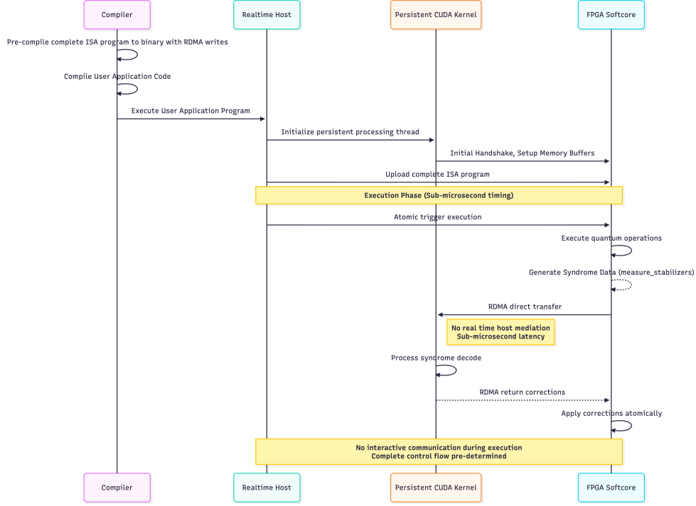
Fig. 6. Sequence diagram describing the interaction between Real-time Host, CUDA Device, and FPGA control to enable realtime data marshaling and classical device callback invocation for systems with short coherence time requirements. Quantum kernels must be compiled ahead-of-time to FPGA-control-specific ISA binary code. The Real-time Host must initialize the total system - launching persistent CUDA threads that wait for FPGA-delivered data for processing.
