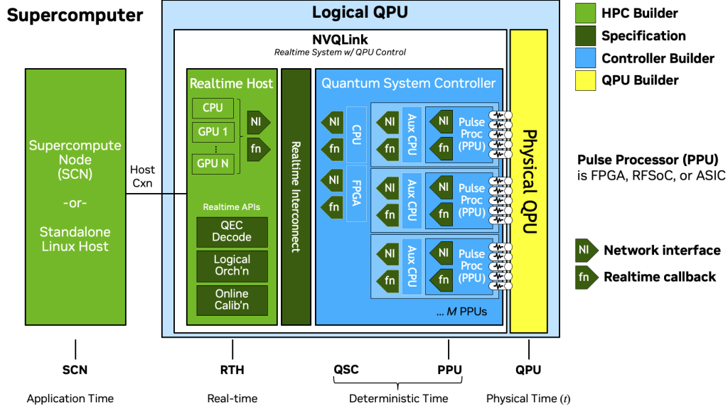
Fig. 1. Machine model of the Logical QPU. The NVQLINK architecture comprises the Real-time Host (RTH) and QPU Control System (QSC) connected by a low-latency, scalable Real-time Interconnect joining them into a network capable of handling the runtime workloads of a Fault Tolerant Quantum Computer. The RTH contains traditional HPC compute resources (CPUs and GPUs and perhaps other specialized hardware), while the QSC contains the Pulse Processing Units controlling the QPU. These compute resources also comprise the key memory and storage resources for the application to consider and orchestrate including GPU memory, RTH system main memory, etc. The programming model for this system is built to recognize all CPUs, GPUs, and resources within the QSC including CPUs, PPU, and other specialized FPGA resources, as targetable Devices and enable Real-time Callback functions (fn) among them to support distributed processing and data marshaling. To support this, a small and optional Network Interface (NI) is provided that enables unilateral and private adoption by the QSC builder. This construction affords flexibility in the value chain of Physical QPU, QSC, and runtime protocols such as QEC Decoding and Online Calibration: each of these components is provided by a third party who may build or integrate some or all of the system and who may share their implementation of each component or keep it proprietary at their discretion. The purpose of this architecture is support such flexibility while enabling every implementation to achieve state-of-the-art HPC performance at minimal cost and time to solution.
