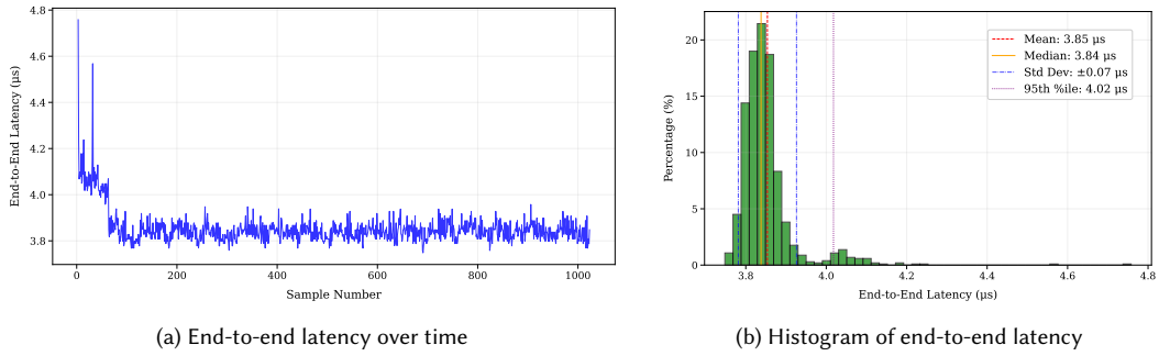
Fig. 4. Observing slight increased warm-up latency at the beginning of a run
