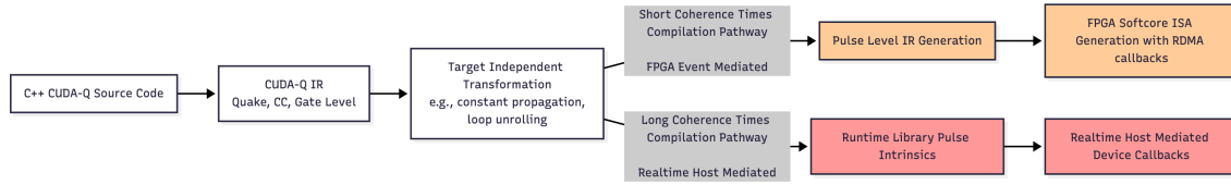
Fig. 8. (top left) Prototypical CUDA-Q quantum kernel code demonstrating quantum code interleaved with realtime classical processing on an NVQLINK device. This code executes on a Logical QPU and compiler code generation depends on the timing domain inherent to the targeted architecture. Compiler implementations, as a first step, should lower to a unified representation that is amenable for further target-specific lowering (top right). Below these snippets (bottom), we see how compiler workflows should approach the proposed system timing domains.
