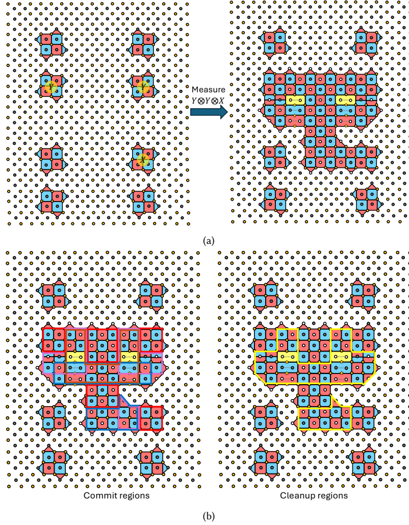
Fig. 9. (a) Example of a logical Y \otimes Y \otimes X measurement implemented via lattice surgery for surface code patches with d = 3 . The yellow vertices correspond to data qubits and grey vertices to ancillas. Red (blue) plaquettes correspond to X ( Z )-type stabilizers. Twist defects are represented by yellow plaquettes. White vertices represent random stabilizer measurements in the first syndrome measurement round when the patches are merged. However the product of all stabilizers with white vertices corresponds to the parity of the Y \otimes Y \otimes X measurement. Stabilizer measurements of the merged surface code patch are measured over d_m rounds, after which data qubits in the routing space region are measured in the X -basis which splits the surface code patches back to their original form. (b) Partitioning of a 2D slice of the merged lattice into commit (red boxes) regions and cleanup regions (yellow boxes). Errors in all commit regions are decoded in parallel. Likewise, errors in all cleanup regions are decoded in parallel. For commit regions, errors are corrected using stabilizer measurements from the red boxes, as well as surrounding buffer regions (shown by blue, purple and brown boxes).
