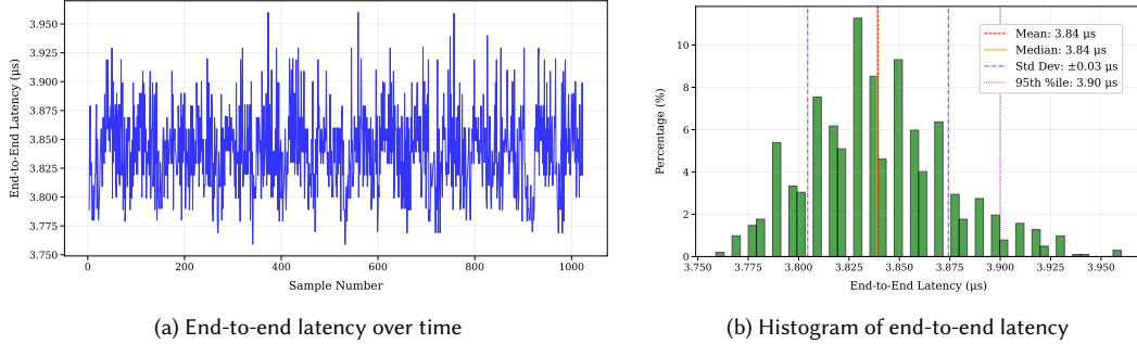
Fig. 5. Steady state latency during the same run as Fig. 4
