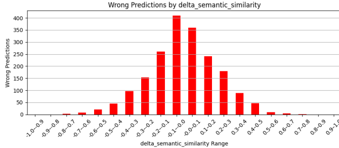
Figure 5: Factor 5 influencing error (Wrong Predictions vs Delta Semantic Similarity)
