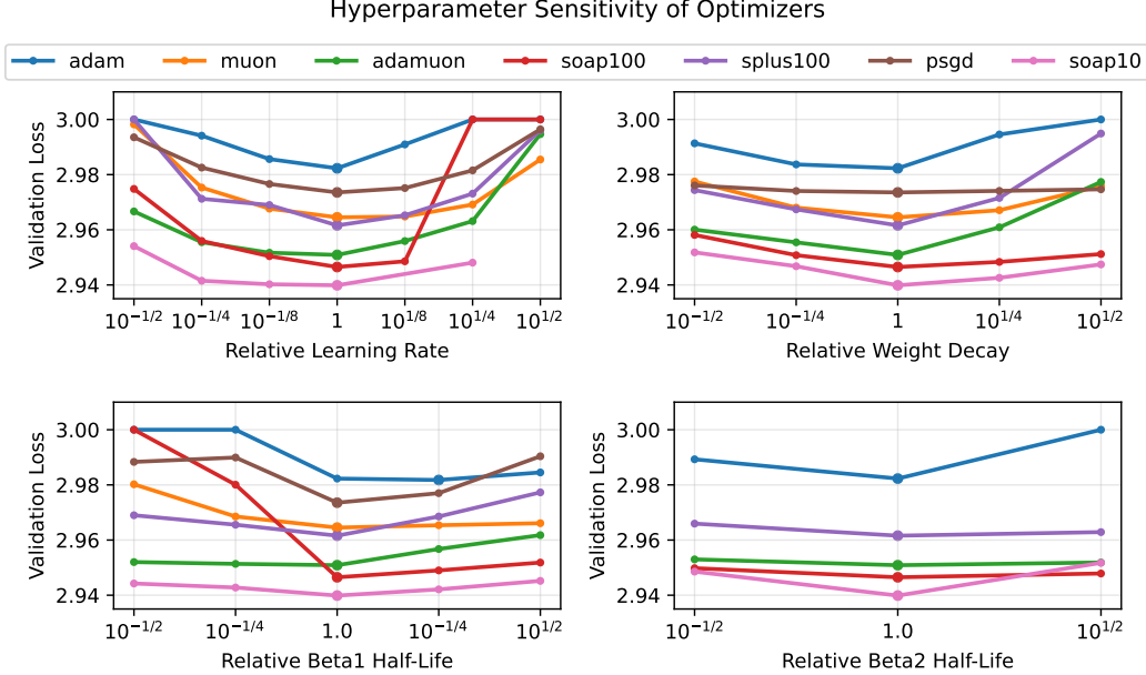
Figure 2: All methods are tuned to within a local optimum of four key hyperparameters. Matrix-whitening optimizers generally maintain their relative performance gains across local adjustments to hyperparameters. Plots are centered around each method’s optimal hyperparameters.
