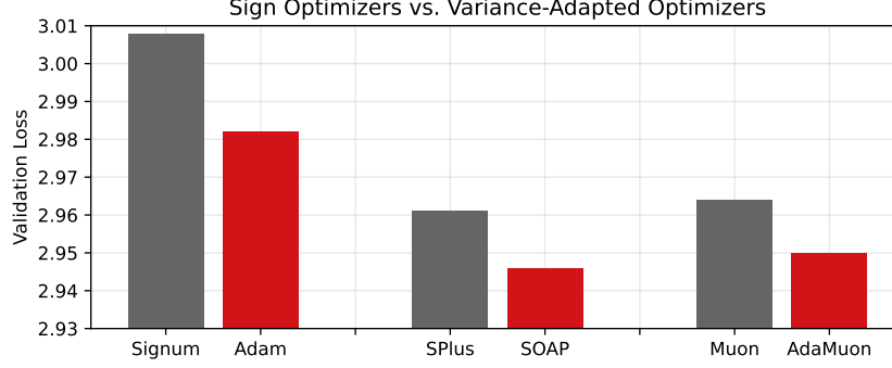
Figure 4: Variance-adapted variants of optimizers outperform their strictly signed-descent counterparts. As elaborated more in Table 3, these improvements remain when the variance buffer is factorized into a rank-1 approximation, as well as to a less degree when \beta_1 = \beta_2 . Variance adaptation can be interpreted as imposing a signal-to-noise dependent adaptive trust region, composable with the rotational or spectral-normalizing aspects of matrix-whitening.
