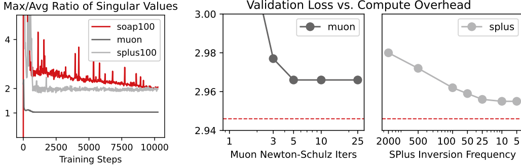
Figure 3: Left: Muon descends under the spectral norm more accurately than SOAP or SPlus. This is achieved when all singular values in the update are \pm 1 , and accordingly the ratio between the maximum and average is close to 1. In contrast, the Shampoo-style methods perform this only loosely, with a ratio between 2 to 3. Adam results in a ratio of \approx 12 (not plotted). Right: Even with increased computation, Muon or SPlus do not reach the empirical performance of SOAP. For Muon, we increase the number of Newton-Schulz iterations at each step. For SPlus, we increase the frequency of updating the eigenbasis. The red dotted line represents the performance of SOAP-100.
