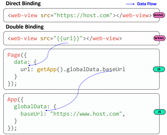
Fig. 6: Data Binding Mechanism in Web-View Domain.
