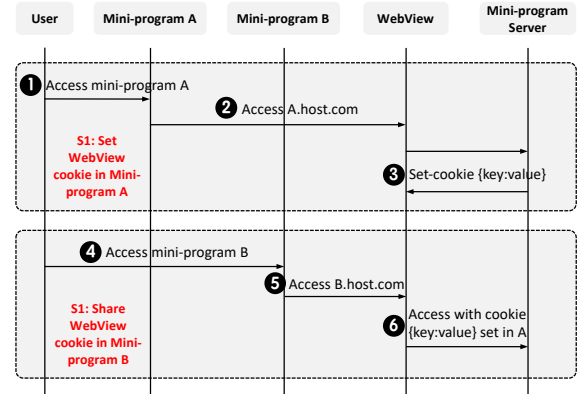
Fig. 1: Cross Mini-program Cookie Sharing via Web-View.
