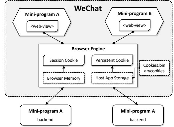
Fig. 3: Design Pitfalls and Root Cause of CMCS.
