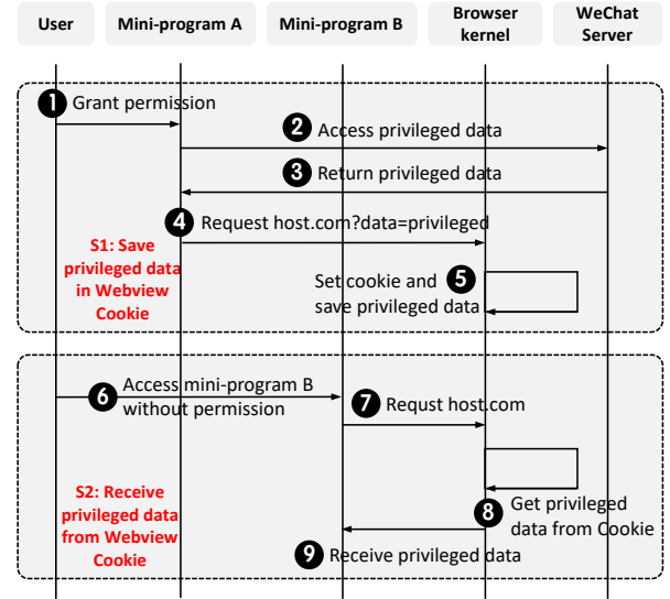
Fig. 4: Collusion Attack via CMCS.
