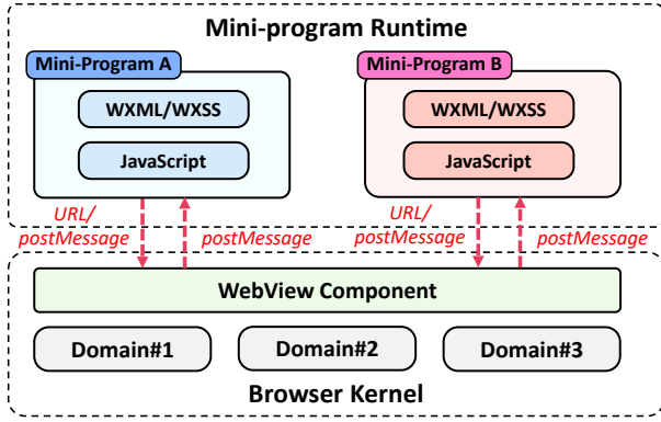
Fig. 2: Architecture of Mini-programs.
